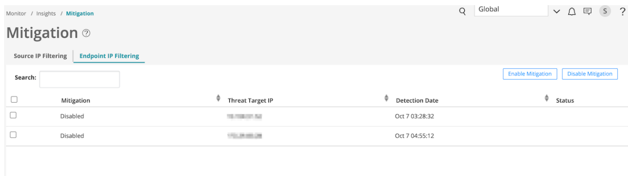
Figure 8: Mitigation Page
