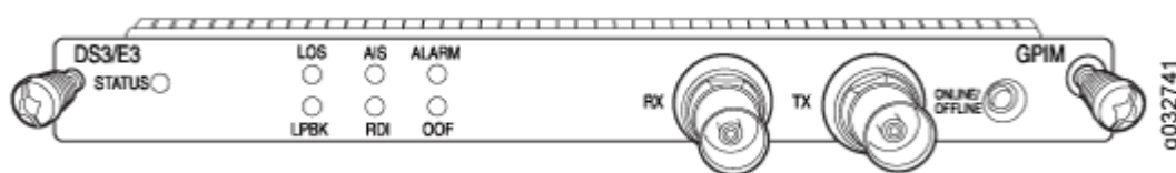
Figure 25: 1-Port Clear Channel DS3/E3 GPIM Front Panel
