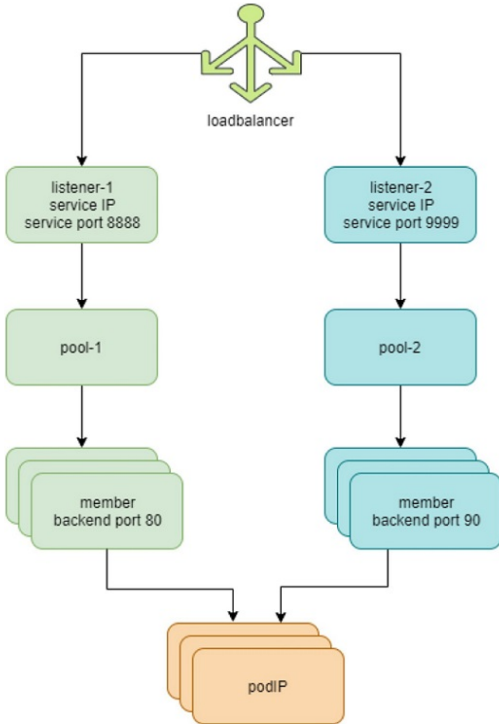
Figure 13: Load Balancer Objects
