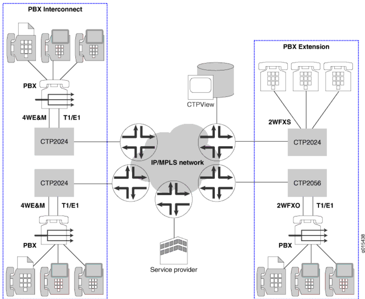
Figure 1: CTP Series Voice Architecture and Key Components
