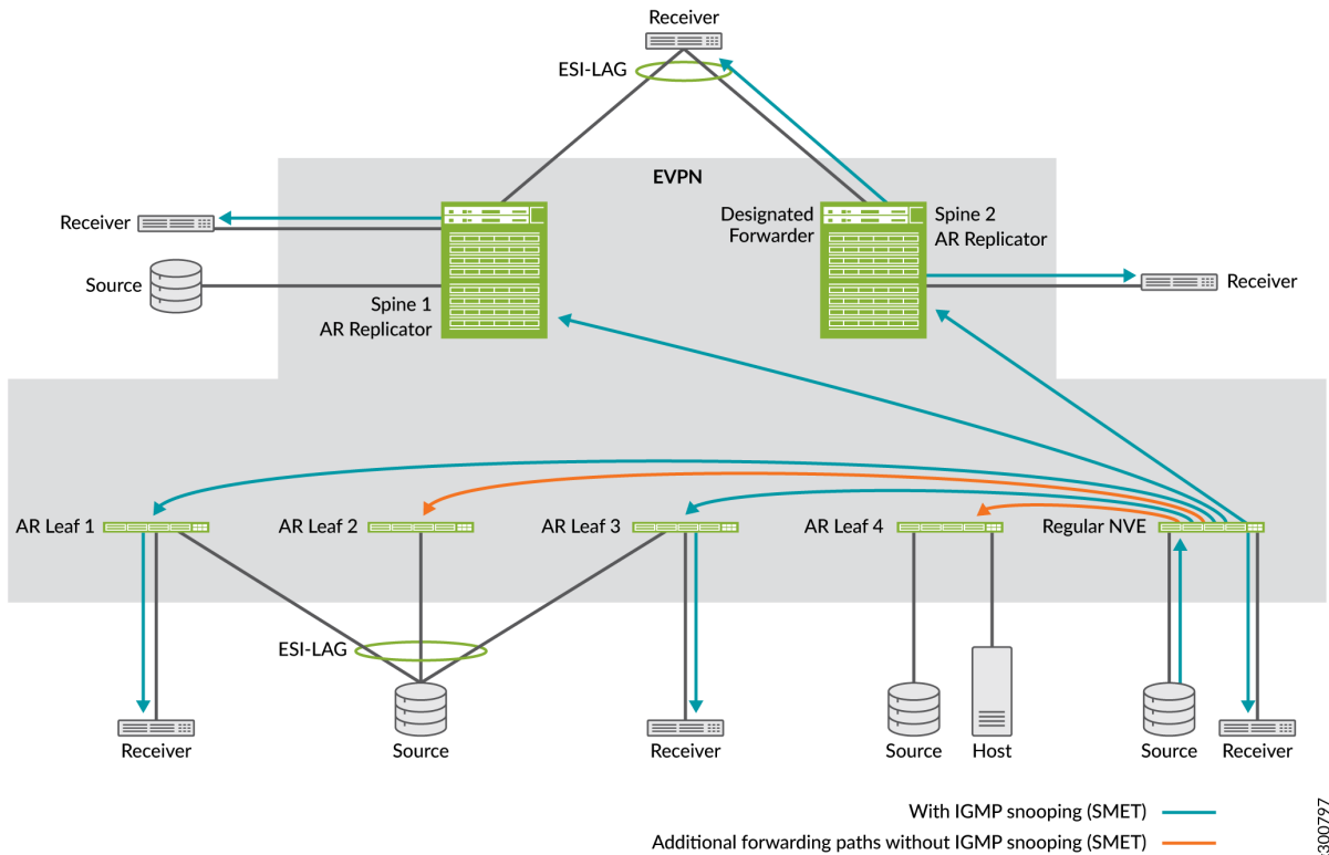
Figure 99: Multicast Source Traffic Ingress at a Regular NVE Device
