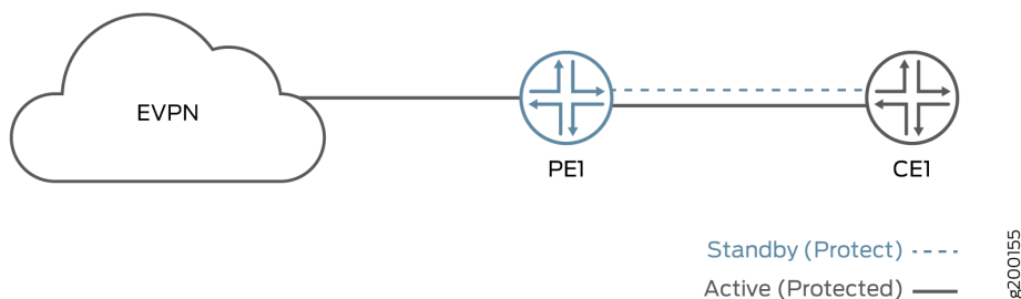
Figure 24: EVPN Active-Standby Multihoming on a Single PE Device
