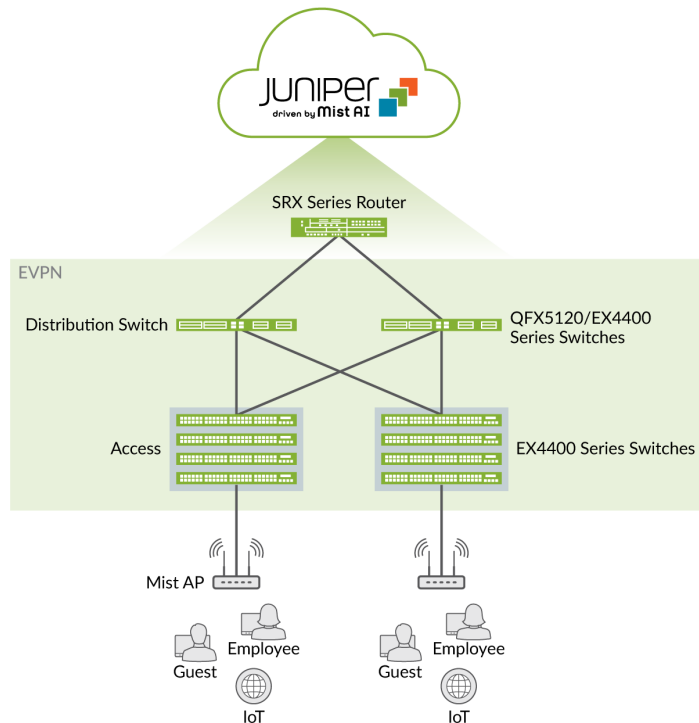
Figure 62: VXLAN GBP on an EX4400 Switch
