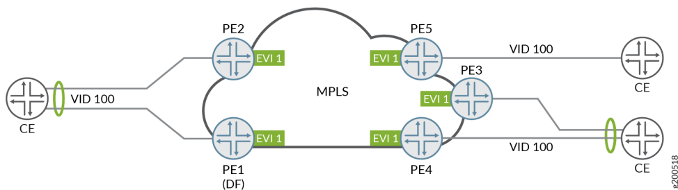
Figure 132: Single VID with no VLAN Translation
