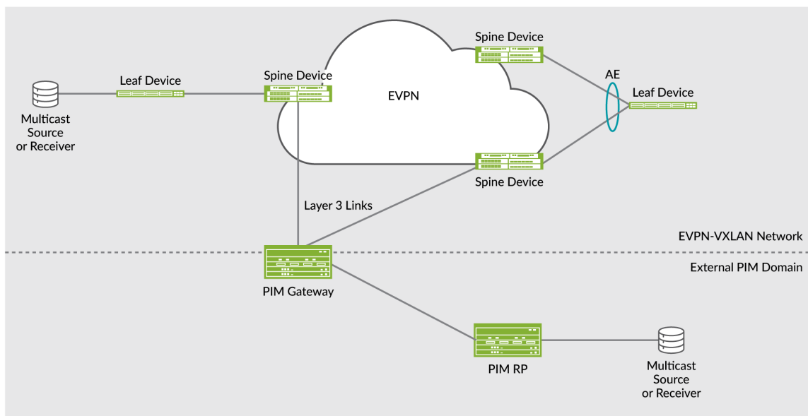
Figure 91: Use Case 4: PIM Gateway with Layer 3 Connectivity—Key Components
