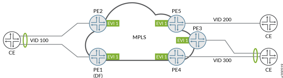
Figure 133: Multiple VIDs with VLAN Translation
