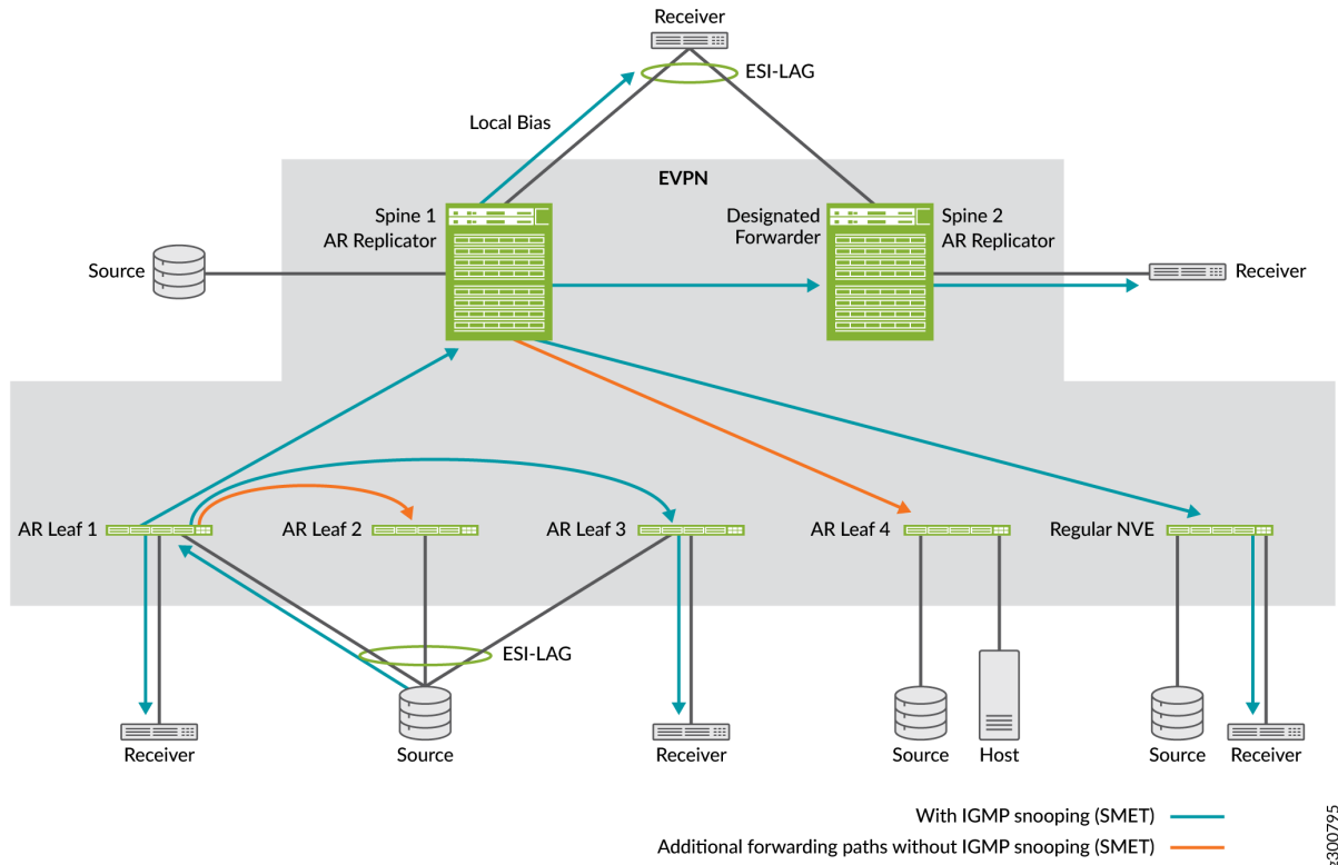
Figure 102: Source Traffic Ingress at an AR Leaf Device (Multihomed Source)
