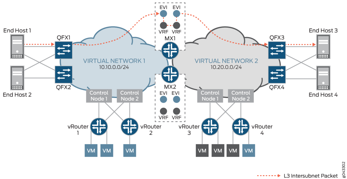
Figure 70: Handling Known Unicast Traffic Between Virtual Networks
