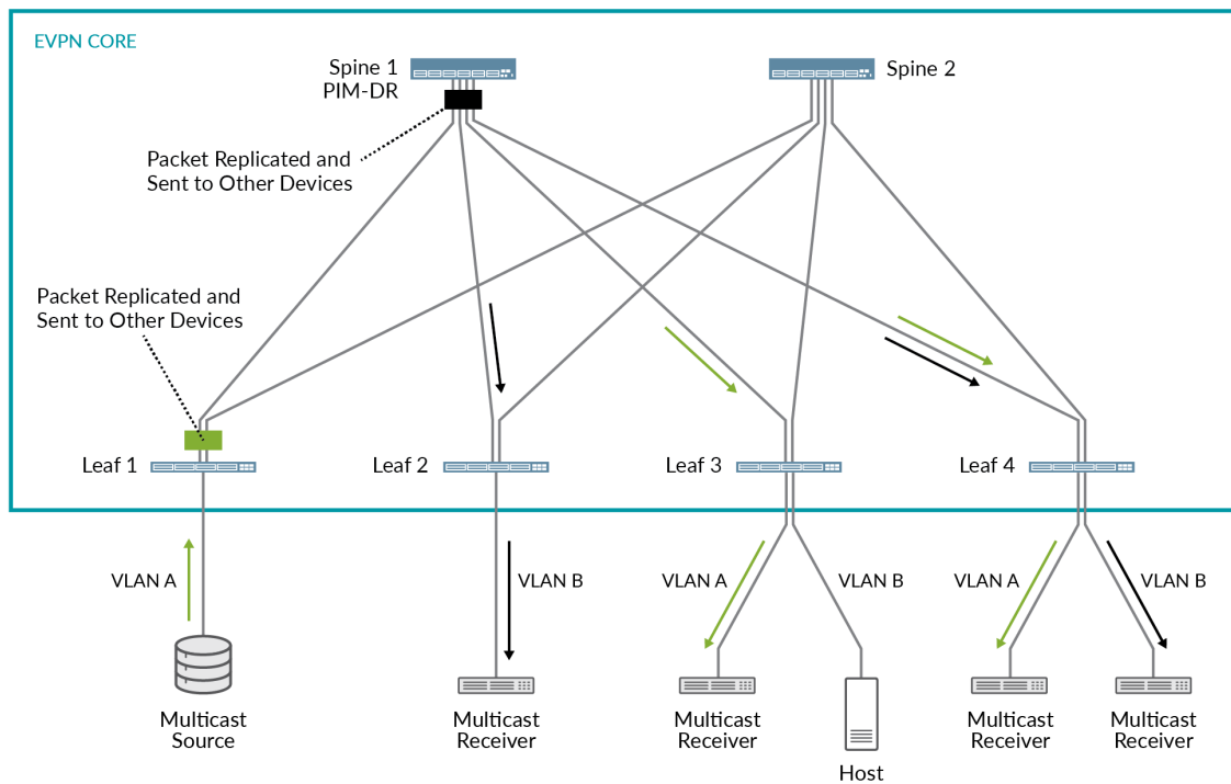
Figure 95: Selective Multicast Forwarding in a Centrally-Routed EVPN-VXLAN Network
