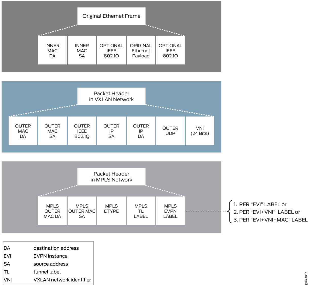
Figure 45: EVPN-VXLAN Packet Format
