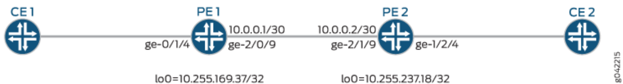
Figure 135: EVPN with Virtual Switch Support
