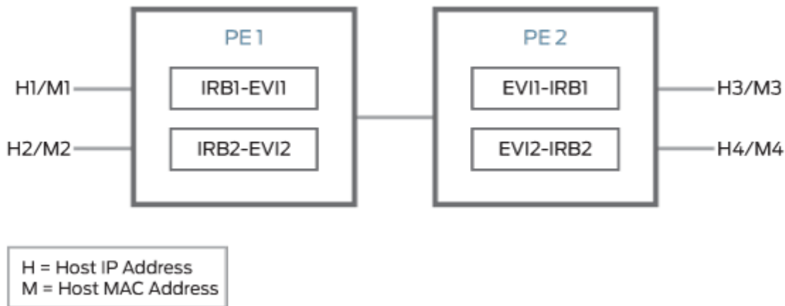
Figure 138: Inter-Subnet Traffic Forwarding
