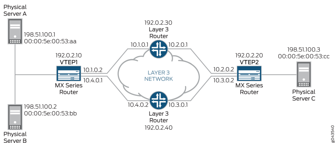
Figure 124: Using Overlay Ping and Traceroute to Troubleshoot a VXLAN
