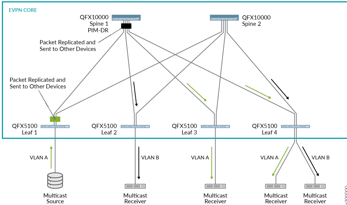
Figure 86: Centrally-Routed Bridging Overlay
