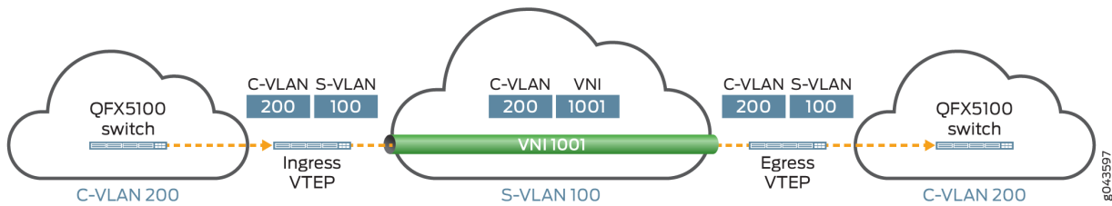
Figure 119: Popping and Later Pushing an S-VLAN Tag
