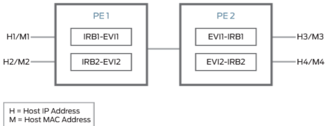
Figure 136: Inter-Subnet Traffic Forwarding
