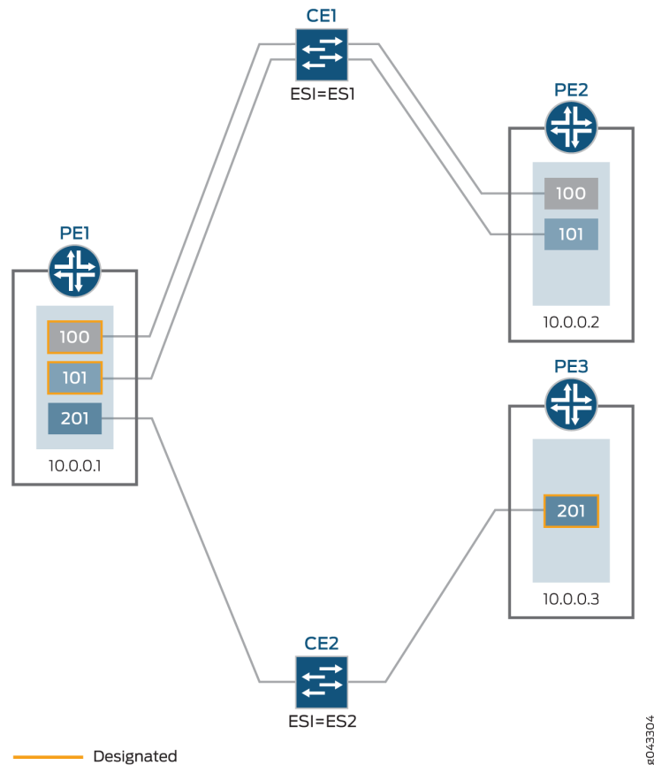
Figure 47: Designated Forwarder Election Topology
