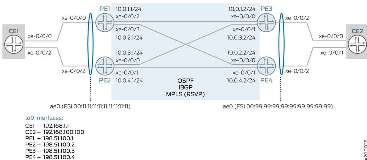
Figure 153: VPWS with EVPN Signaling
