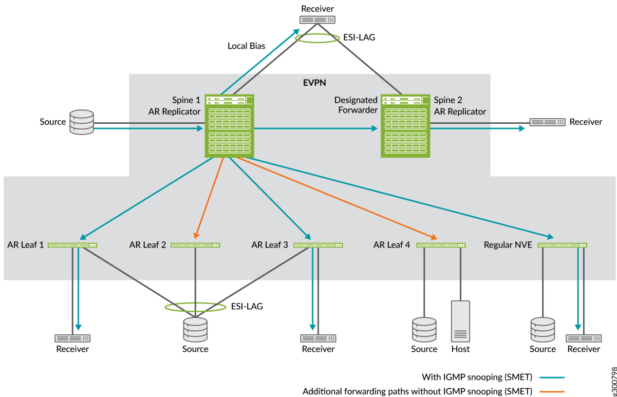
Figure 100: Multicast Source Traffic Ingress at an AR Replicator Device
