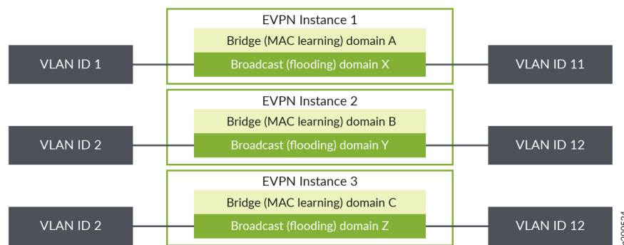
Figure 129: VLAN-Based Service
