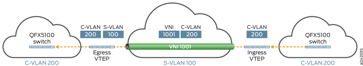
Figure 117: Mapping a Range of C-VLANs to an S-VLAN
