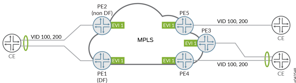
Figure 134: VLAN Bundle Network Topology
