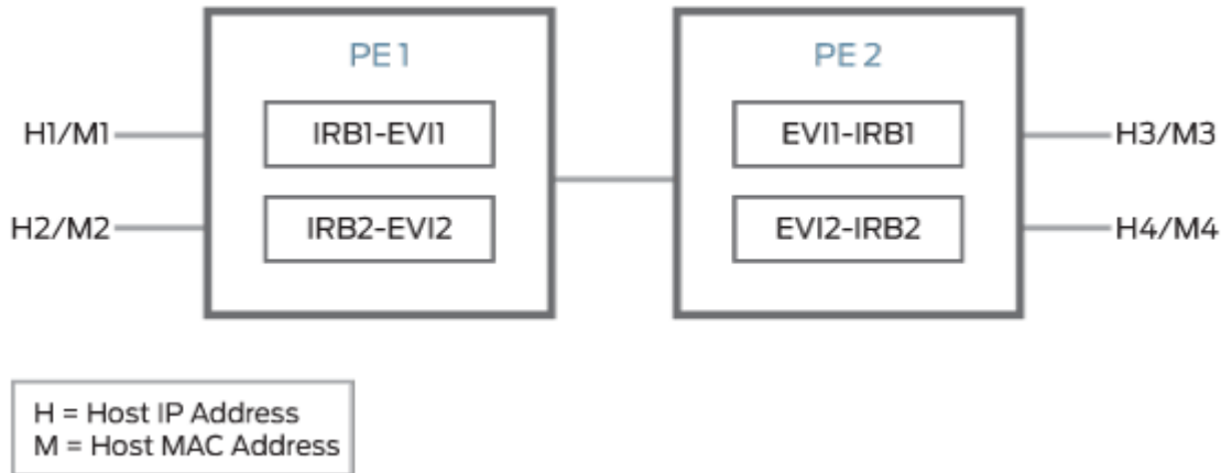
Figure 137: Inter-Subnet Traffic Forwarding
