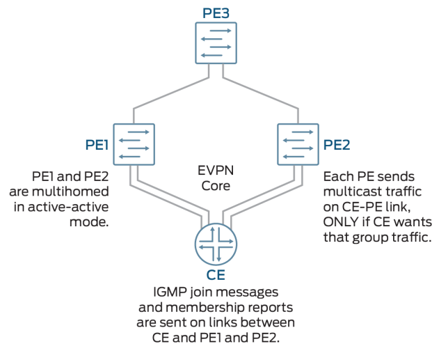
Figure 93: IGMP Snooping in an EVPN-VXLAN Environment
