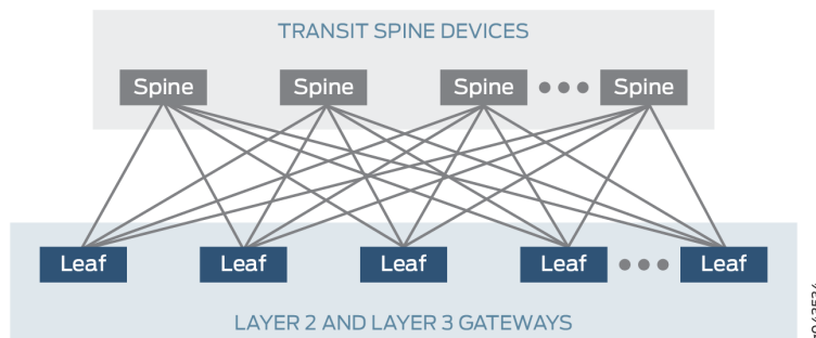
Figure 78: A 3-Stage (Leaf-And-Spine) Edge-Routing Bridging Architecture
