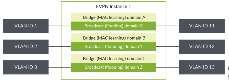
Figure 131: VLAN-Aware Bundle Service
