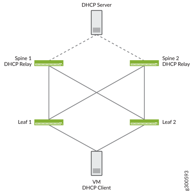
Figure 40: DHCP Relay Agent on Centrally-Routed Bridging Overlay
