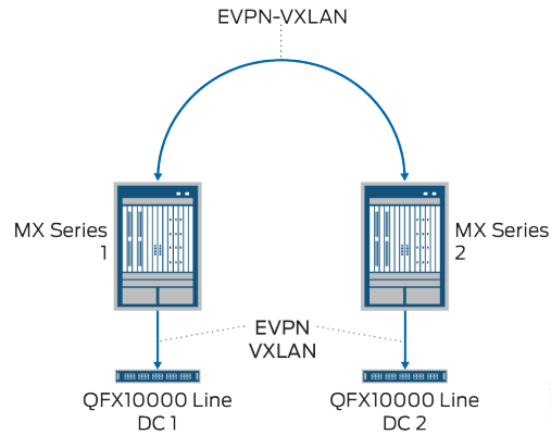
Figure 51: DCI Option: EVPN-VXLAN over the Internet
