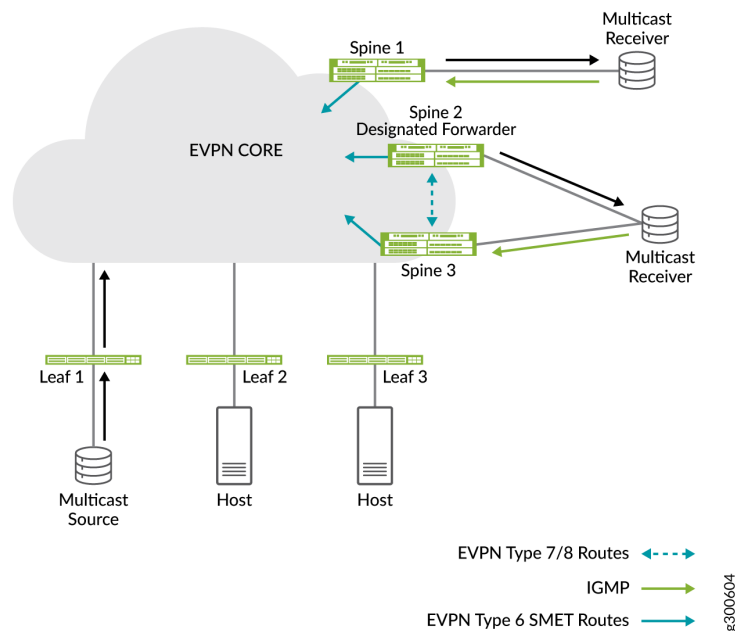
Figure 88: Intra-VLAN Multicast Traffic Flow with IGMP Snooping and Selective Multicast Forwarding
