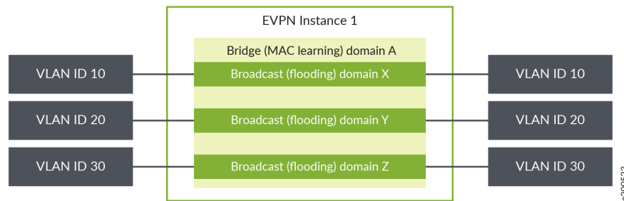
Figure 130: VLAN Bundle Service
