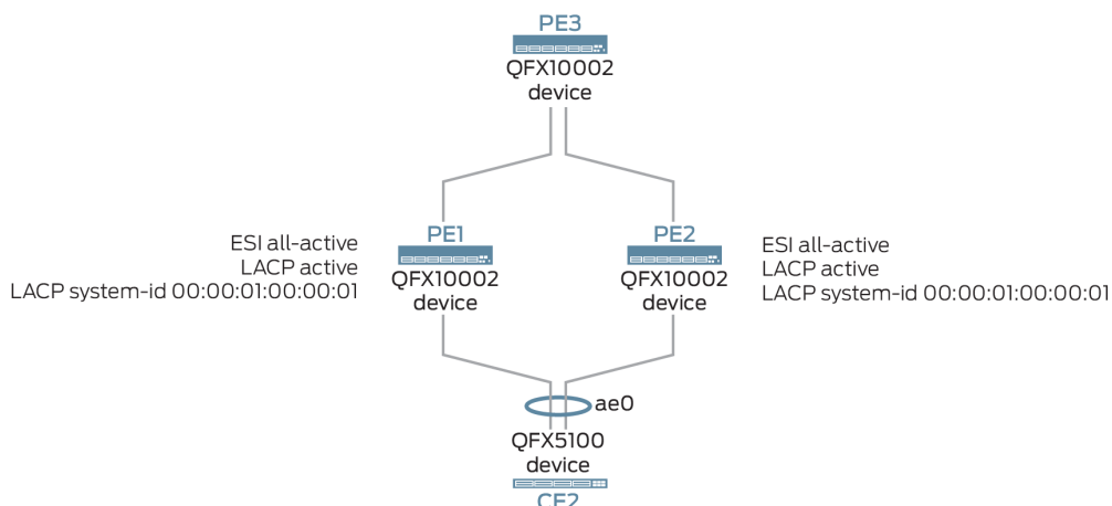
Figure 30: LACP Support in EVPN Active-Active Multihoming
