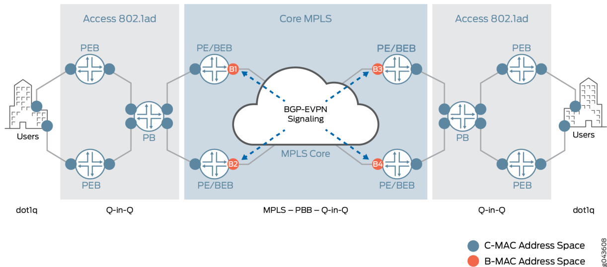
Figure 184: PBB-EVPN Integration
