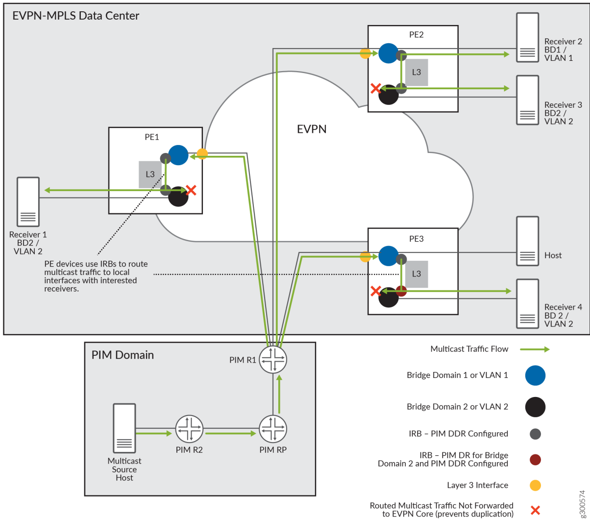
Figure 145: Routing External PIM Domain Source Traffic Between Bridge Domains (or VLANs) with IRBs and PIM DDR in EVPN-MPLS
