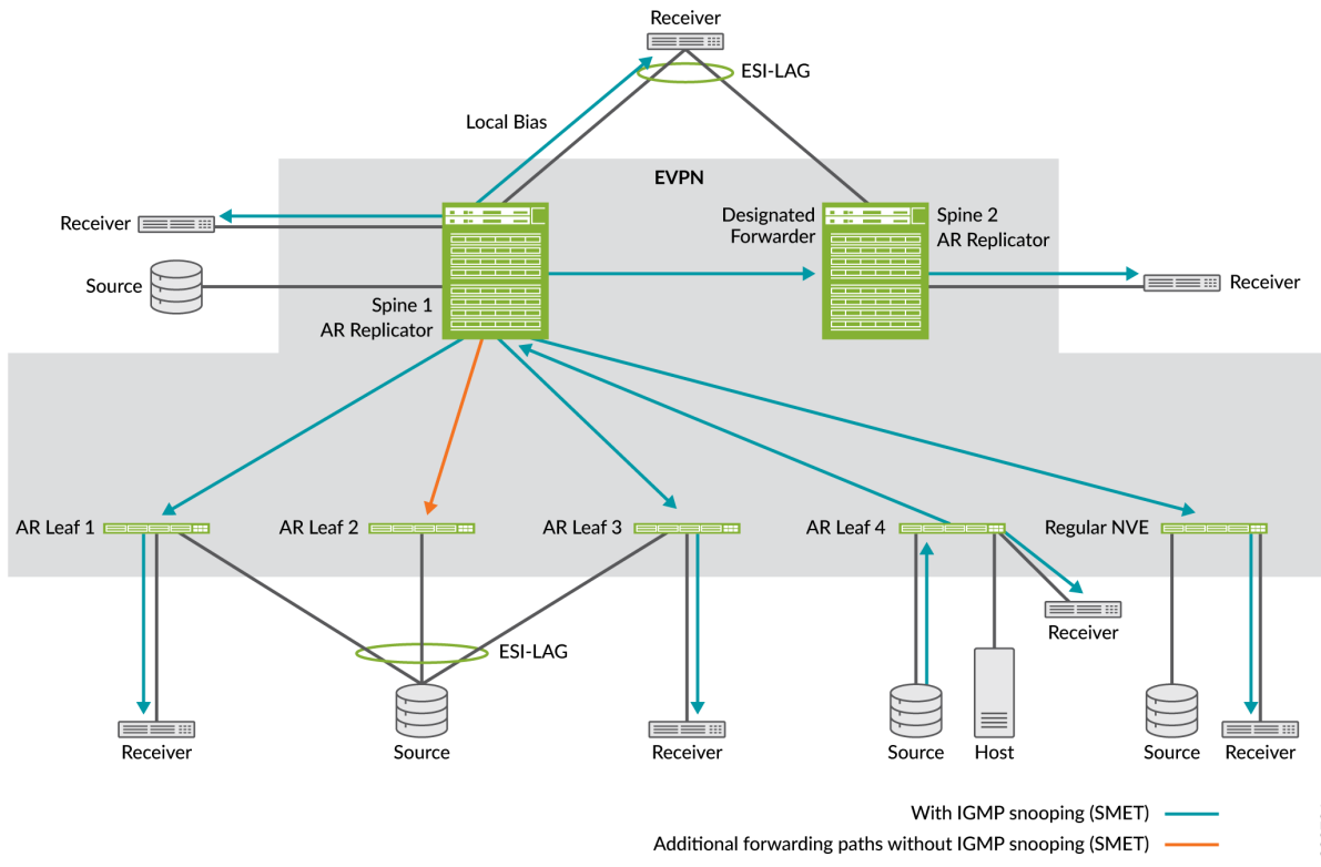
Figure 101: Source Traffic Ingress at an AR Leaf Device (Single-Homed Source)
