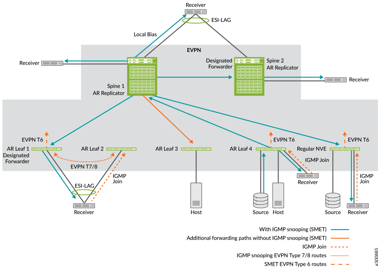
Figure 96: AR Traffic Flow
