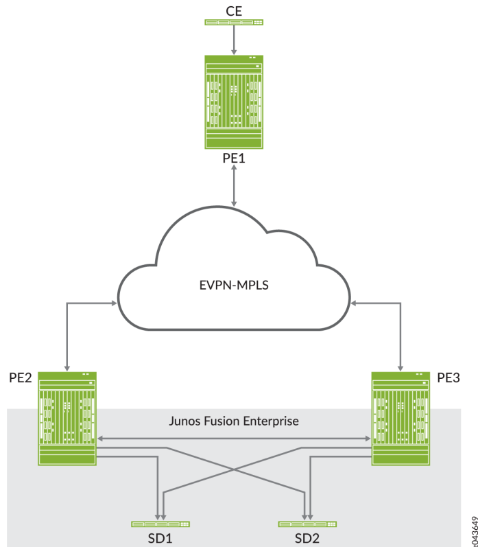
Figure 176: EVPN-MPLS Interworking with Junos Fusion Enterprise
