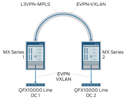
Figure 49: DCI Option: Layer 3 VPN-MPLS
