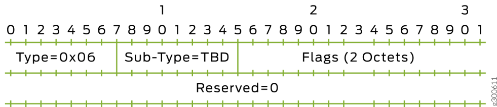
Figure 92: EVPN Multicast Flag Extended Community
