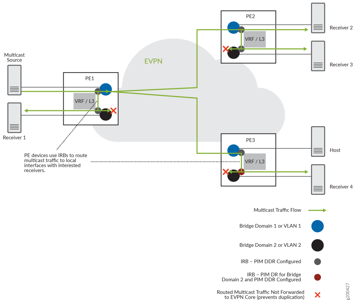
Figure 144: Routing Multicast Traffic Between Bridge Domains (or VLANs) with IRBs and PIM DDR in EVPN-MPLS
