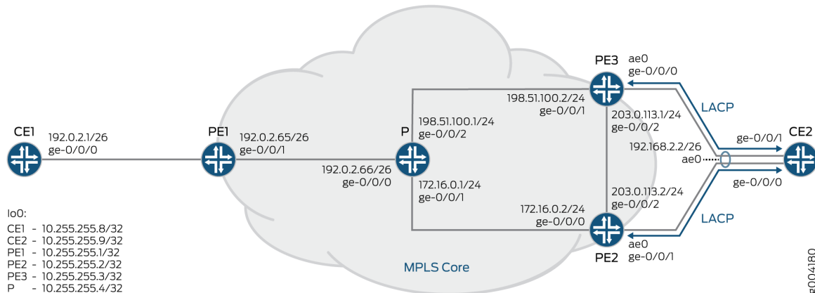
Figure 29: LACP Support in EVPN Active-Active Multihoming
