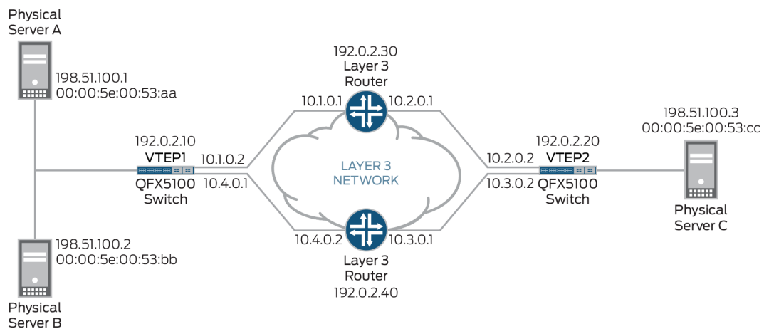
Figure 123: Using Overlay Ping and Traceroute to Troubleshoot a VXLAN Overlay Network
