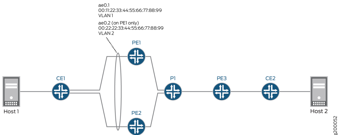
Figure 32: EVPN-MPLS Topology with Multihoming Active-Active
