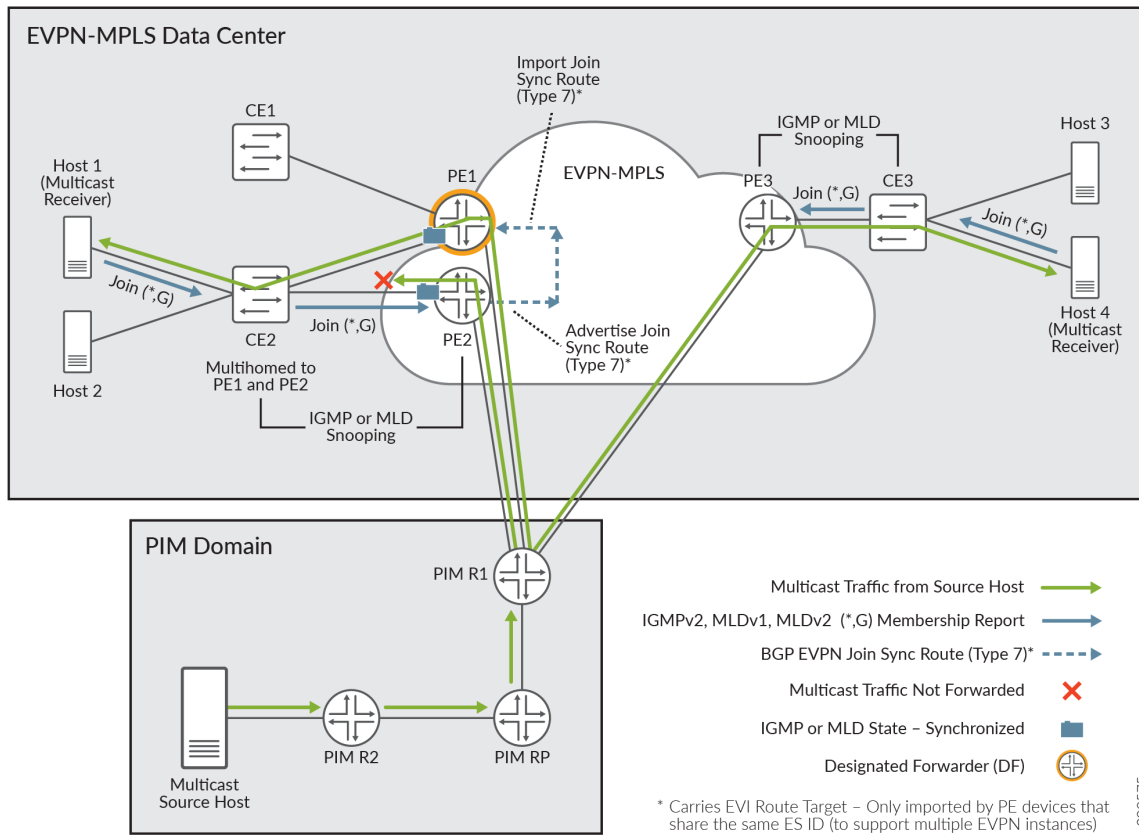
Figure 141: Multicast Forwarding for Multihomed Receivers in EVPN-MPLS on ACX Series Routers
