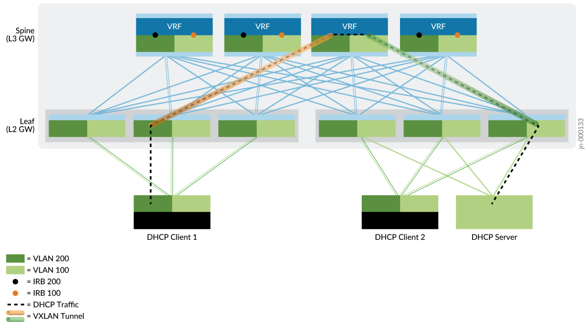
Figure 41: DHCP Relay Agent on Centrally-Routed Bridging Overlay
