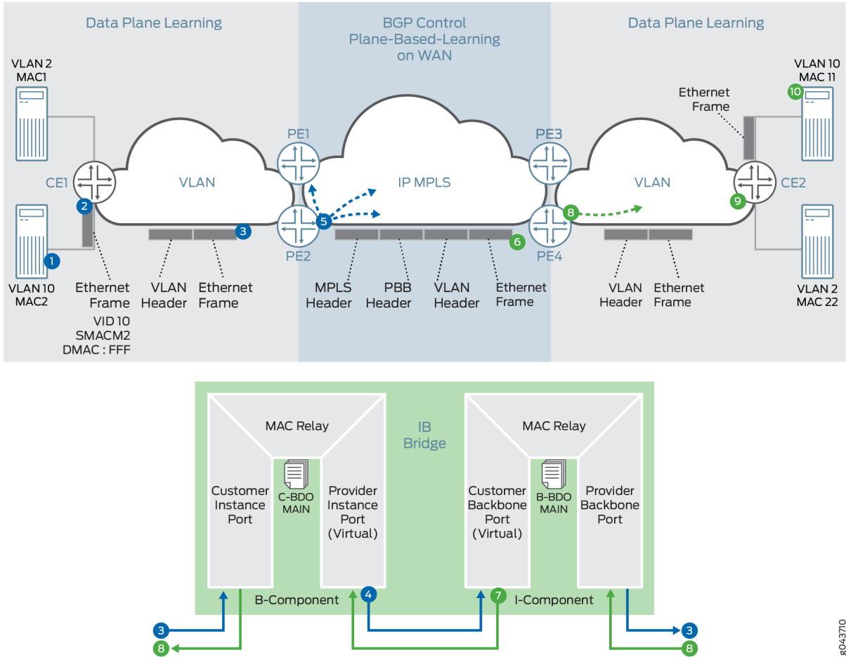
Figure 186: VPN Autodiscovery
