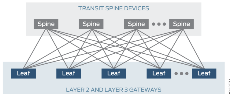
Figure 80: A 3-Stage (Leaf and Spine) Edge-Routing Bridging Architecture
