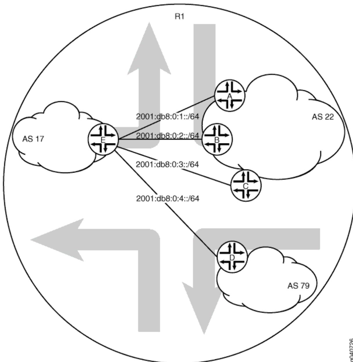
Figure 16: Typical Network with BGP Peer Sessions
