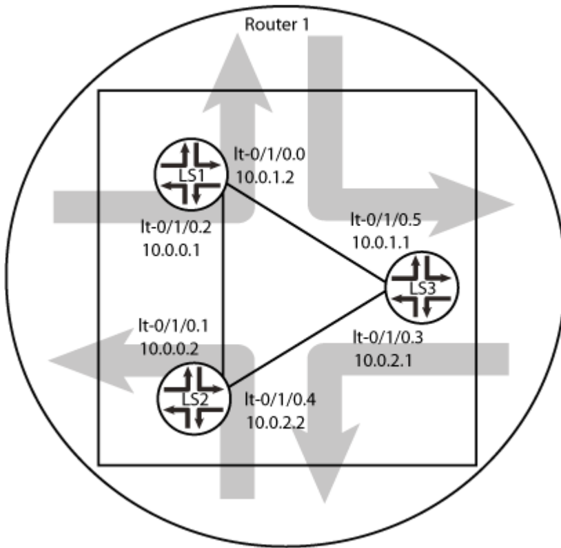
Figure 19: IS-IS on Logical Systems
