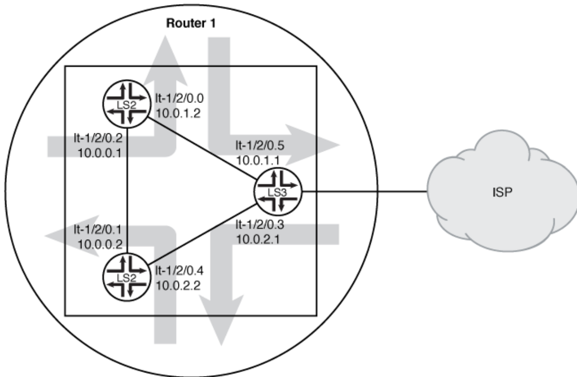
Figure 20: IS-IS with a Default Route to an ISP
