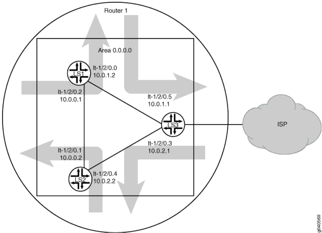
Figure 22: OSPF with a Default Route to an ISP
