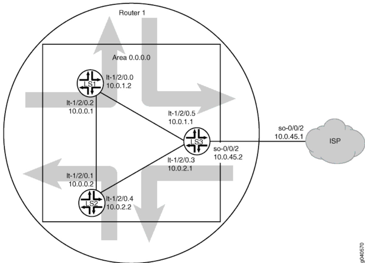
Figure 23: OSPF with a Conditional Default Route to an ISP
