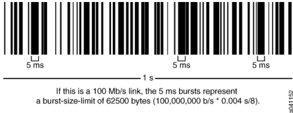
Figure 83: Network Traffic and Burst Rates
