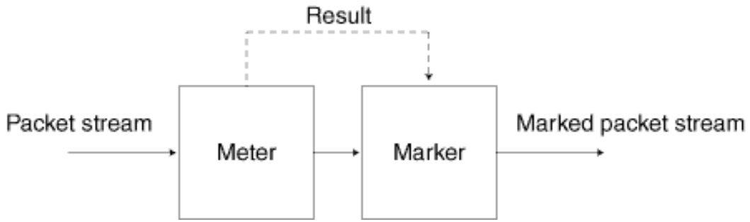
Figure 89: Flow of Tricolor Marking Policer Operation
