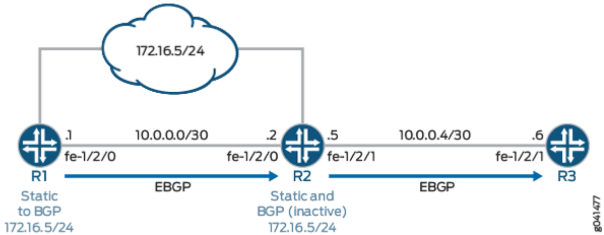
Figure 10: BGP Topology for advertise-inactive
