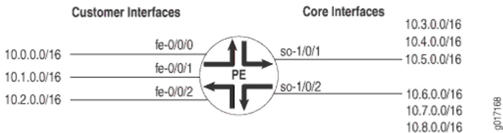
Figure 38: DCU/SCU Concept
