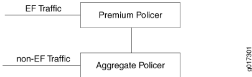
Figure 88: Hierarchical Policer
