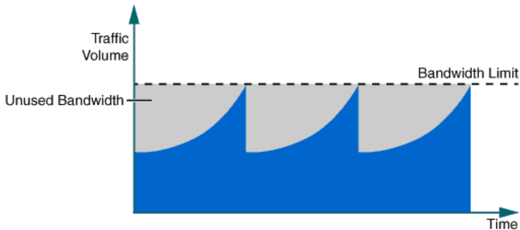
Figure 78: Policer Behavior with a Single TCP Connection
