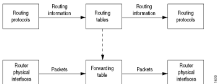
Figure 47: Flows of Routing Information and Packets
