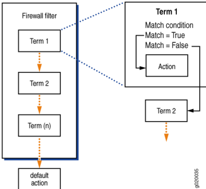
Figure 70: Evaluation of Terms Within a Firewall Filter
