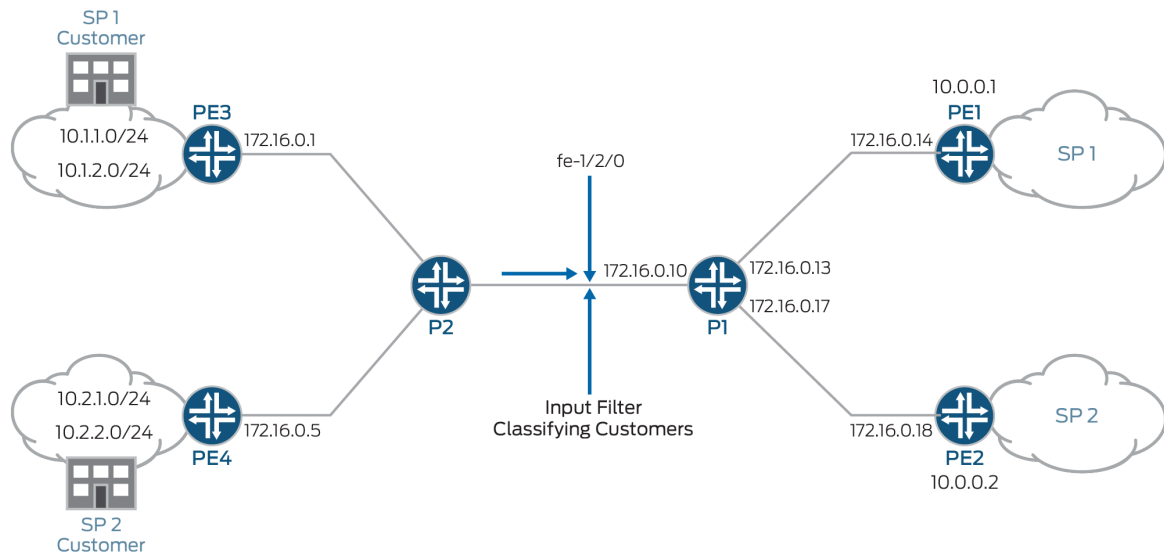
Figure 66: Filter-Based Forwarding
