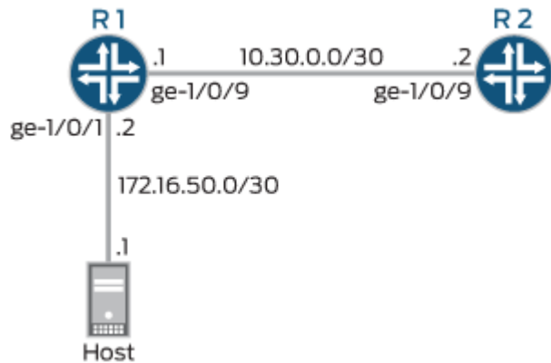
Figure 59: Multifield Classifier Scenario
