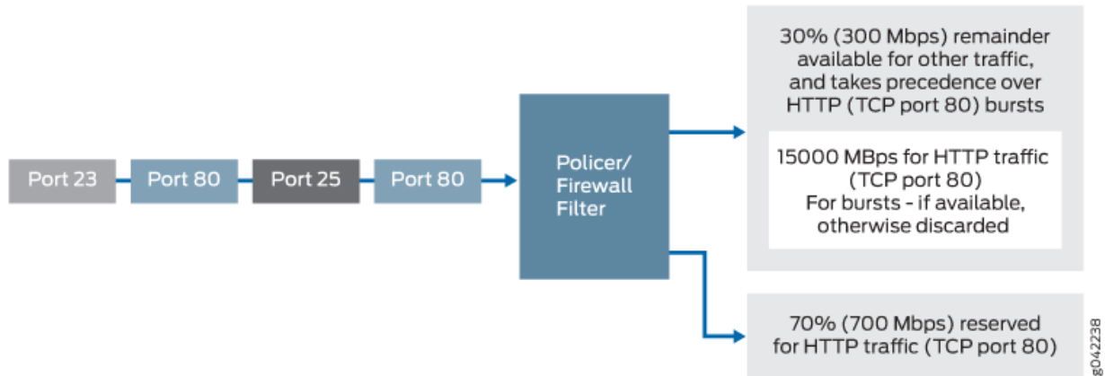
Figure 87: Traffic Limiting in a Single-Rate Two-Color Policer Scenario
