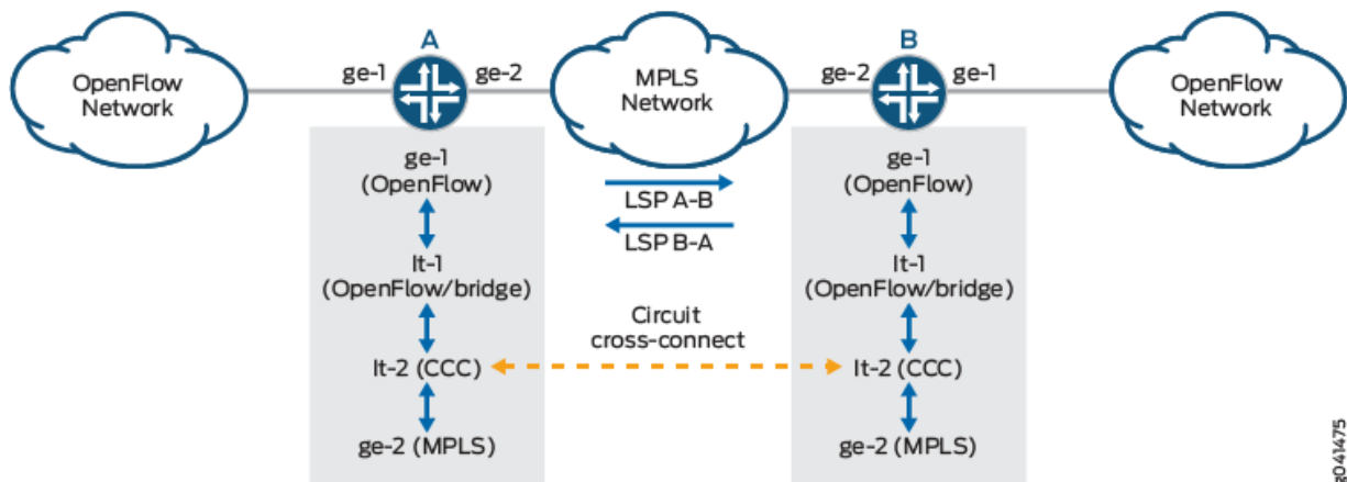
Figure 1: Connecting OpenFlow Networks Using MPLS LSP Tunnel Cross-Connects
