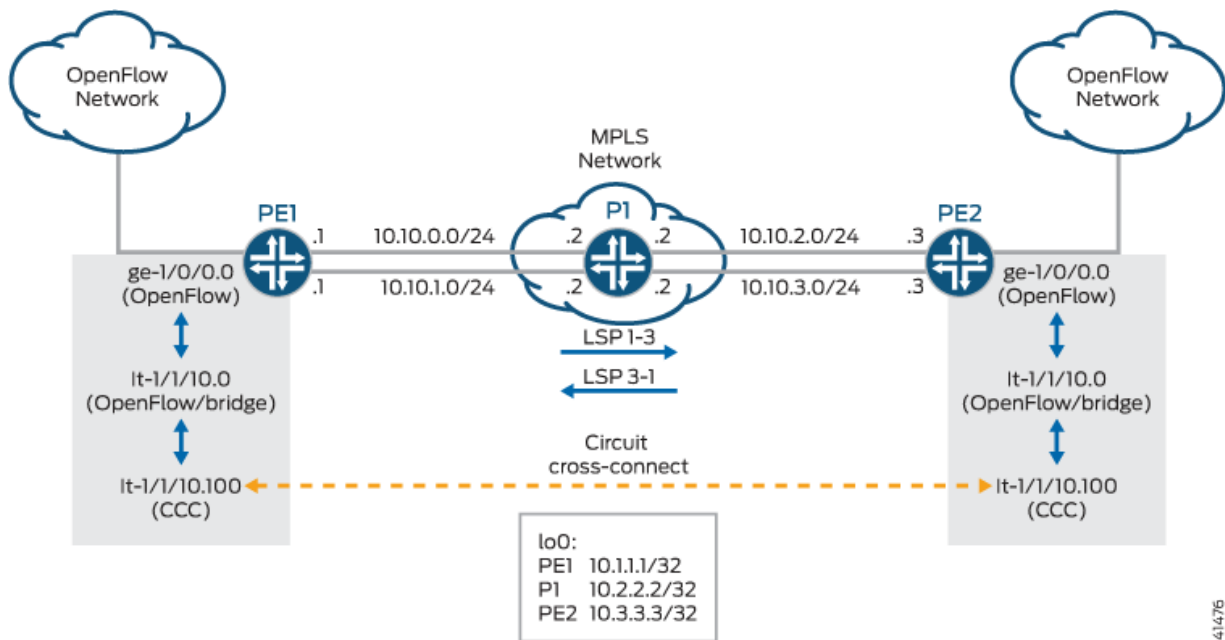
Figure 2: Connecting OpenFlow Networks Using MPLS Tunnel Cross-Connects
