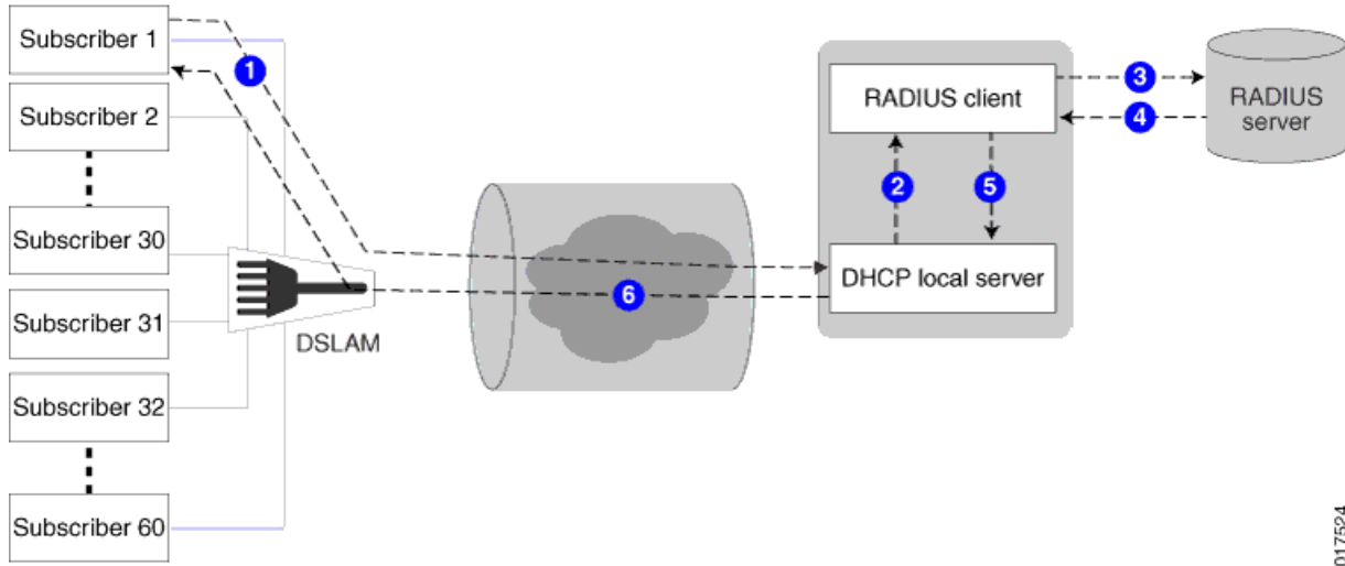
Figure 7: DHCP Options Data Flow
