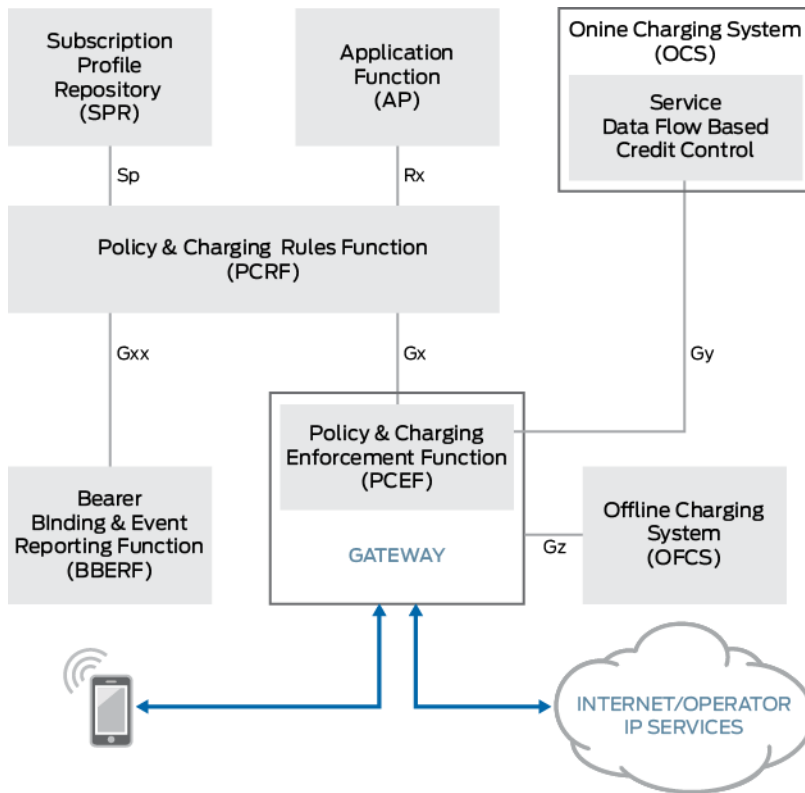
Figure 53: 3GPP PCC Architecture Overview
