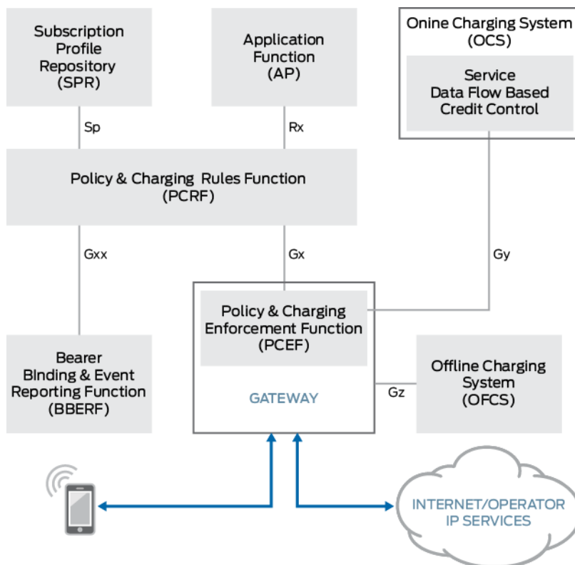
Figure 52: 3GPP PCC Architecture Overview
