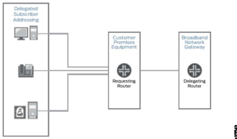
Figure 10: Delegated Addressing in a Dual-Stack Network Using DHCPv6
