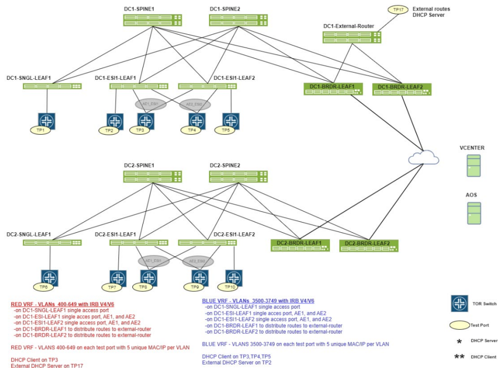
Figure 1: Reference Topology
