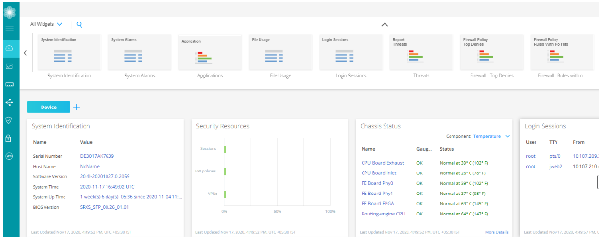
Figure 18: SRX345 Dashboard
