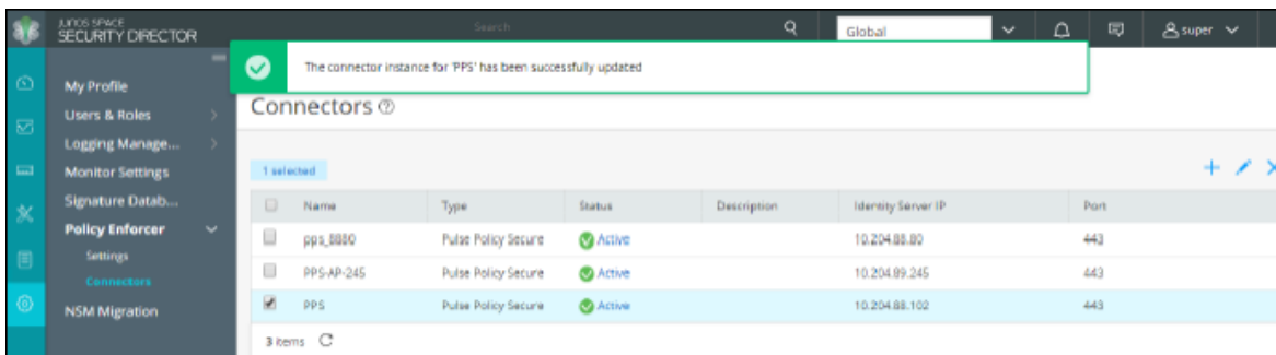
Figure 148: Connectors Page
