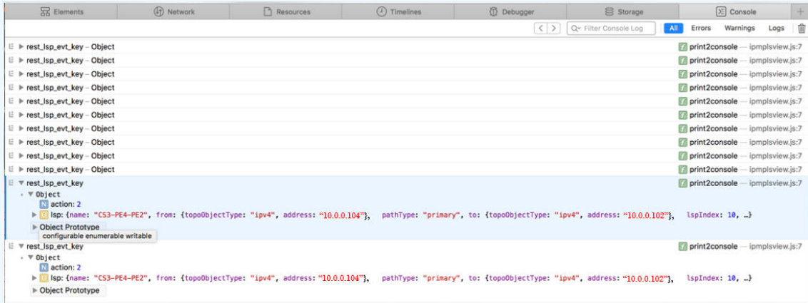
Figure 288: Web Browser Console with Debugging Messages
