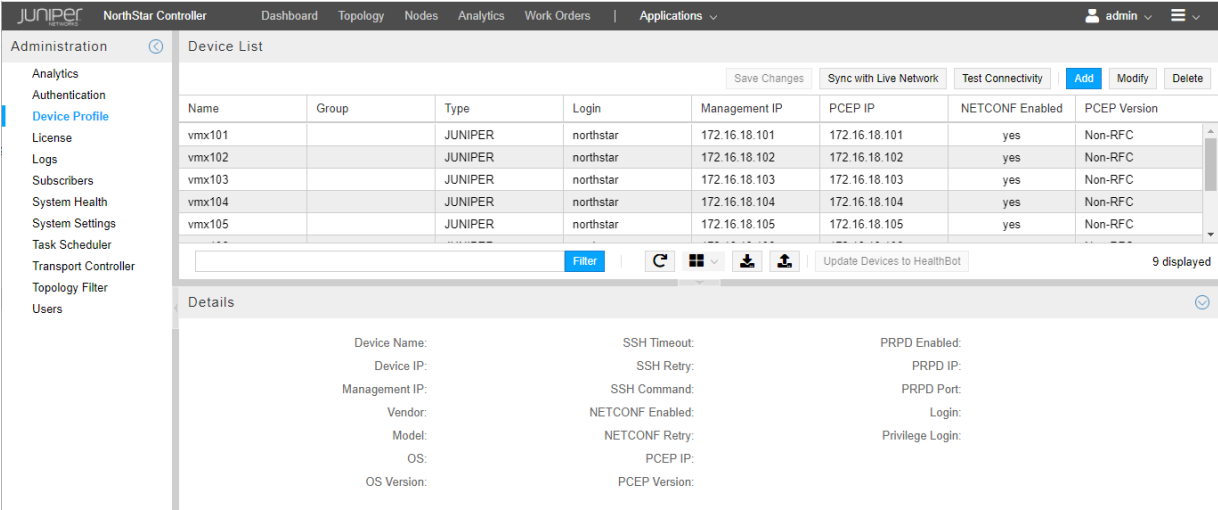
Figure 192: Device Profile Window
