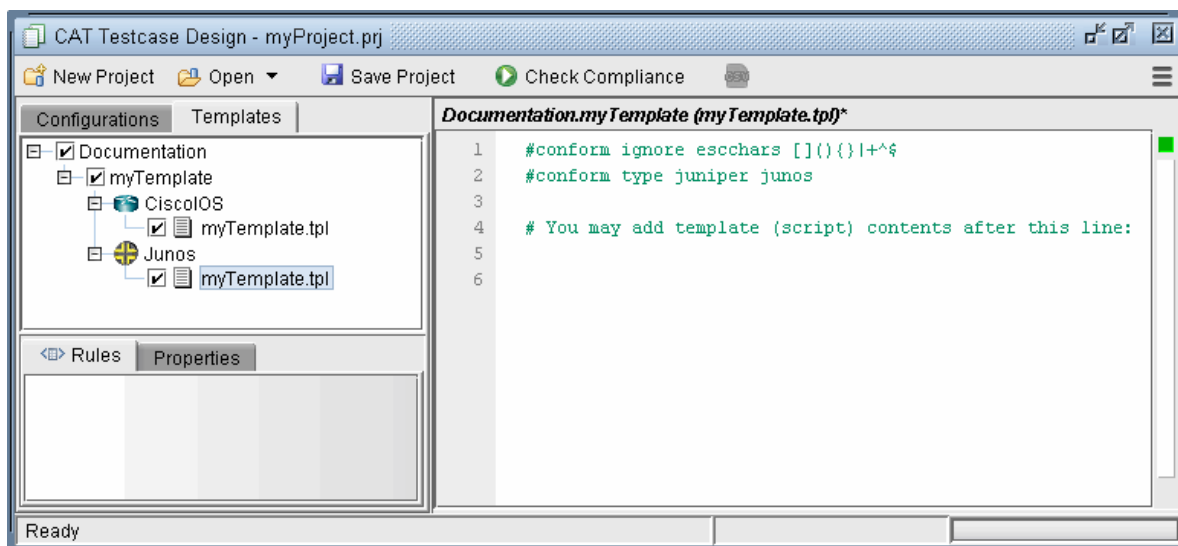
Figure 361: Initial Template
