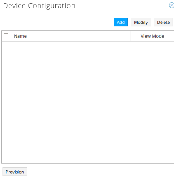
Figure 12: Device Configuration
