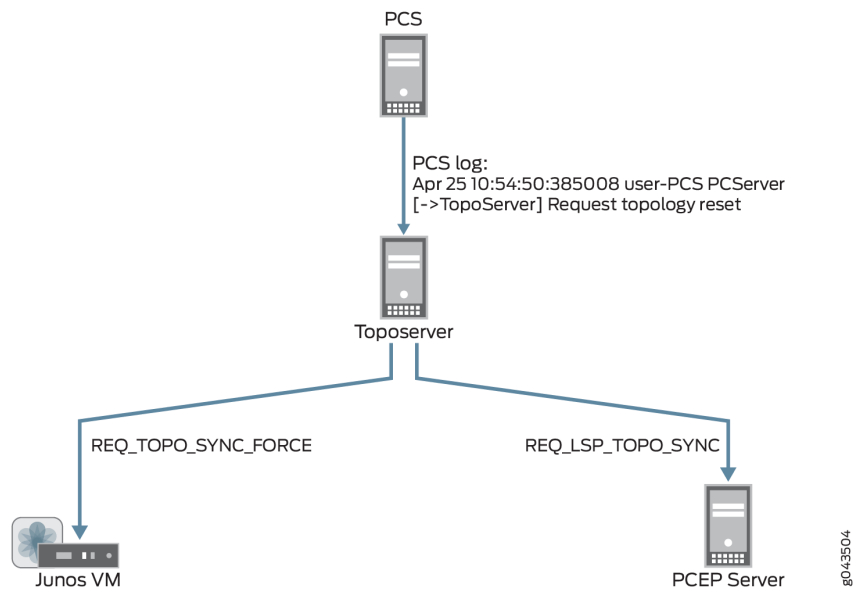
Figure 287: Reset Model Request
