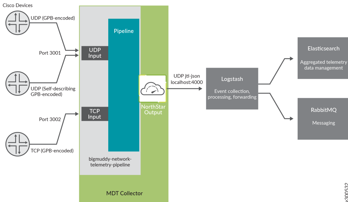
Figure 232: NorthStar MDT Collector Data Flow
