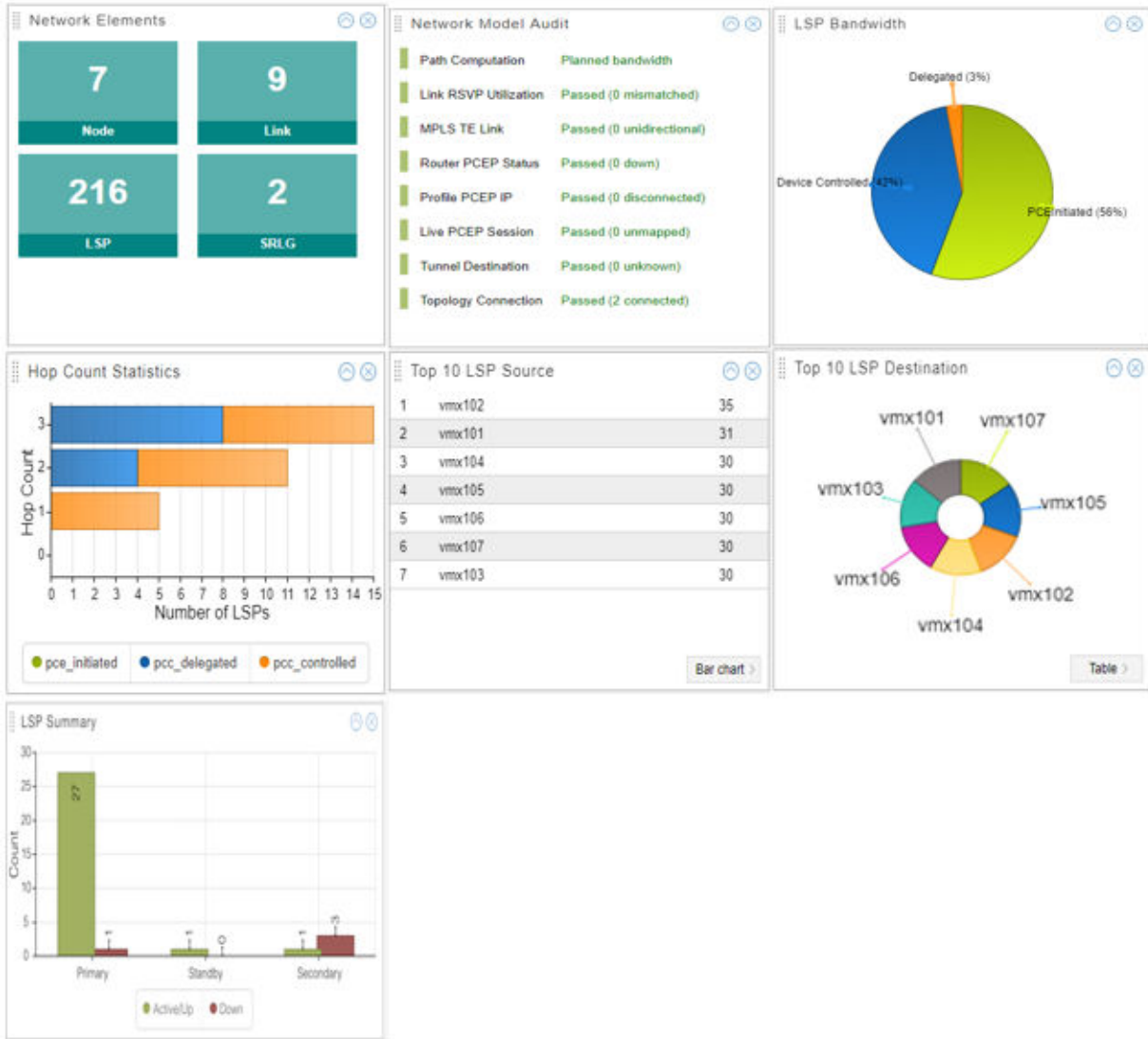
Figure 169: Dashboard Widgets, Not All Showing the Same Network
