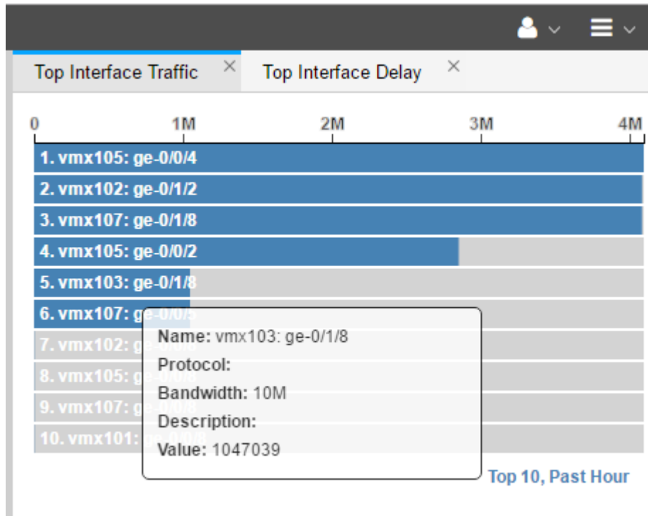
Figure 225: Top Traffic With Mouseover Information
