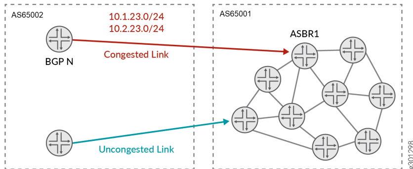
Figure 145: IPE Use Case
