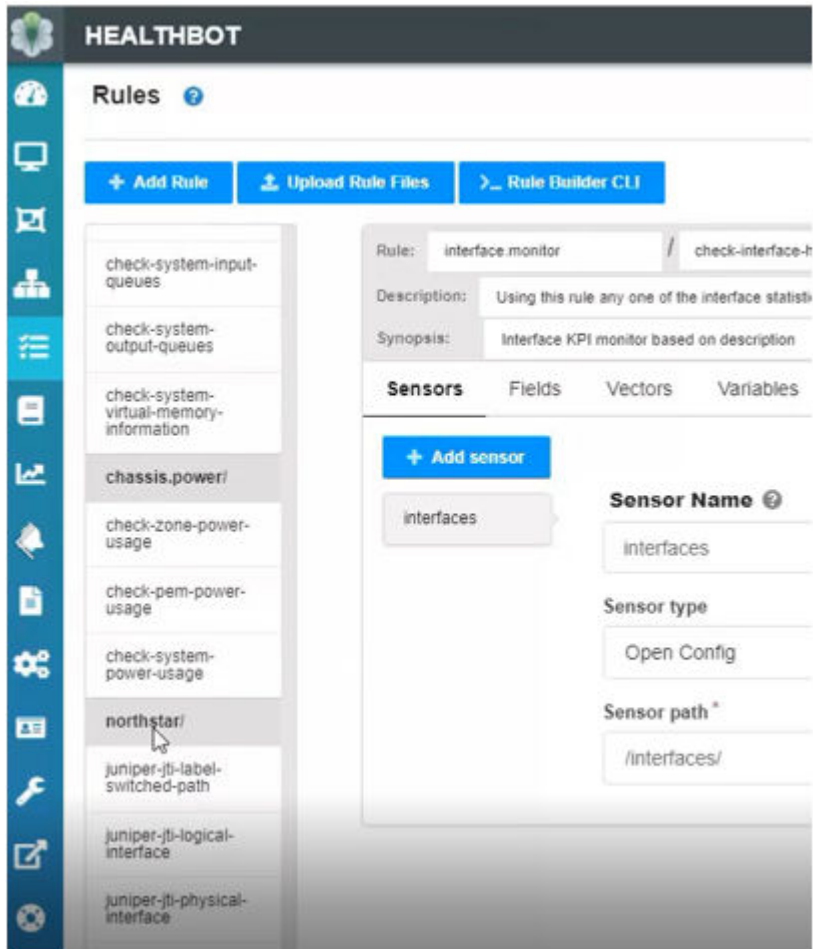
Figure 263: NorthStar Rules in the HealthBot UI
