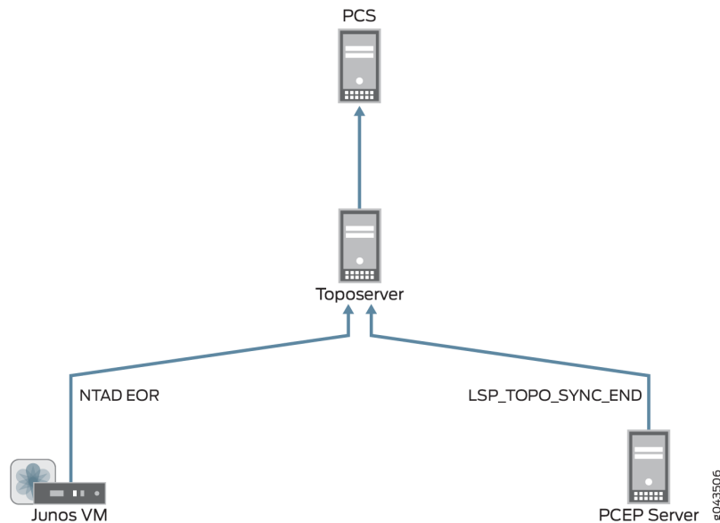
Figure 287: Model Updates Using Reset Network Model
