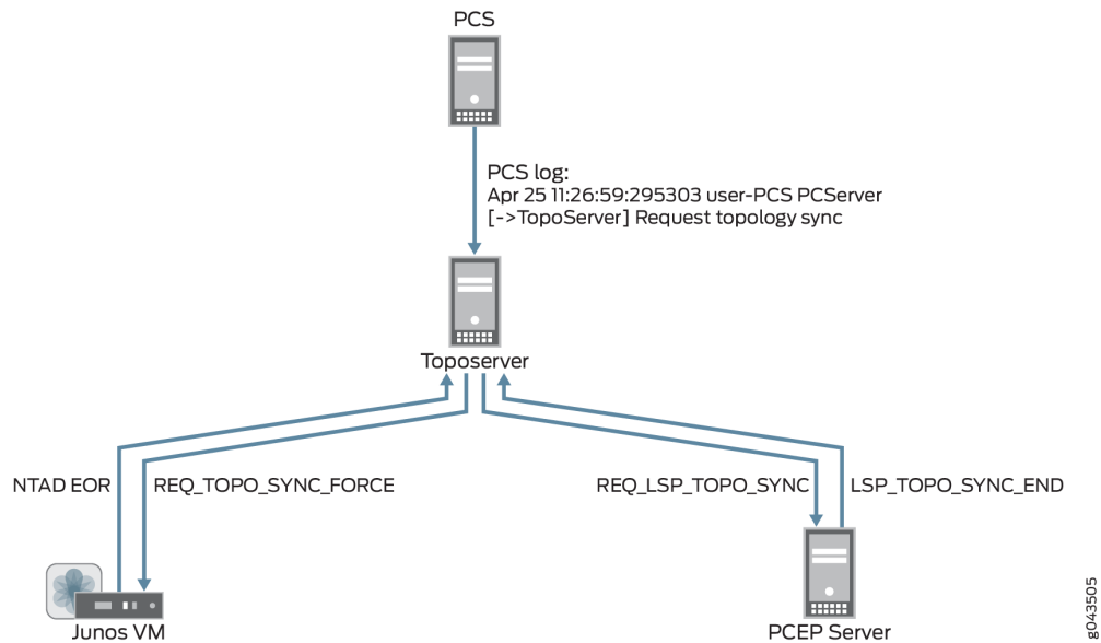
Figure 288: Synchronization Request and Model Updates Using Sync Network Model
