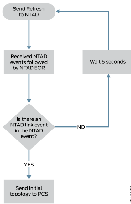
Figure 283: Logic Process for Initial Topology Creation
