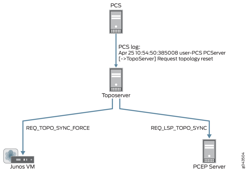
Figure 286: Reset Model Request
