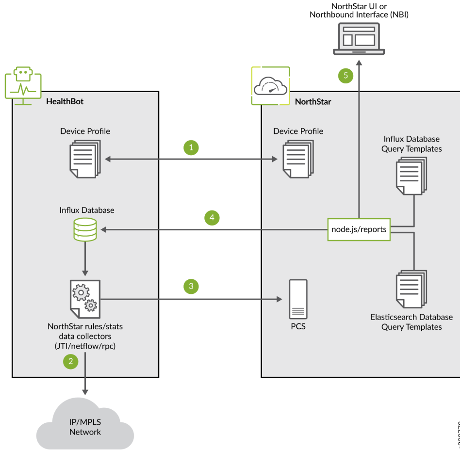
Figure 261: NorthStar Controller/HealthBot Integration
