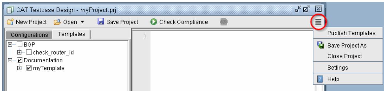
Figure 361: Action menu
