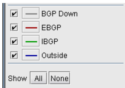
Figure 52: Types Subview
