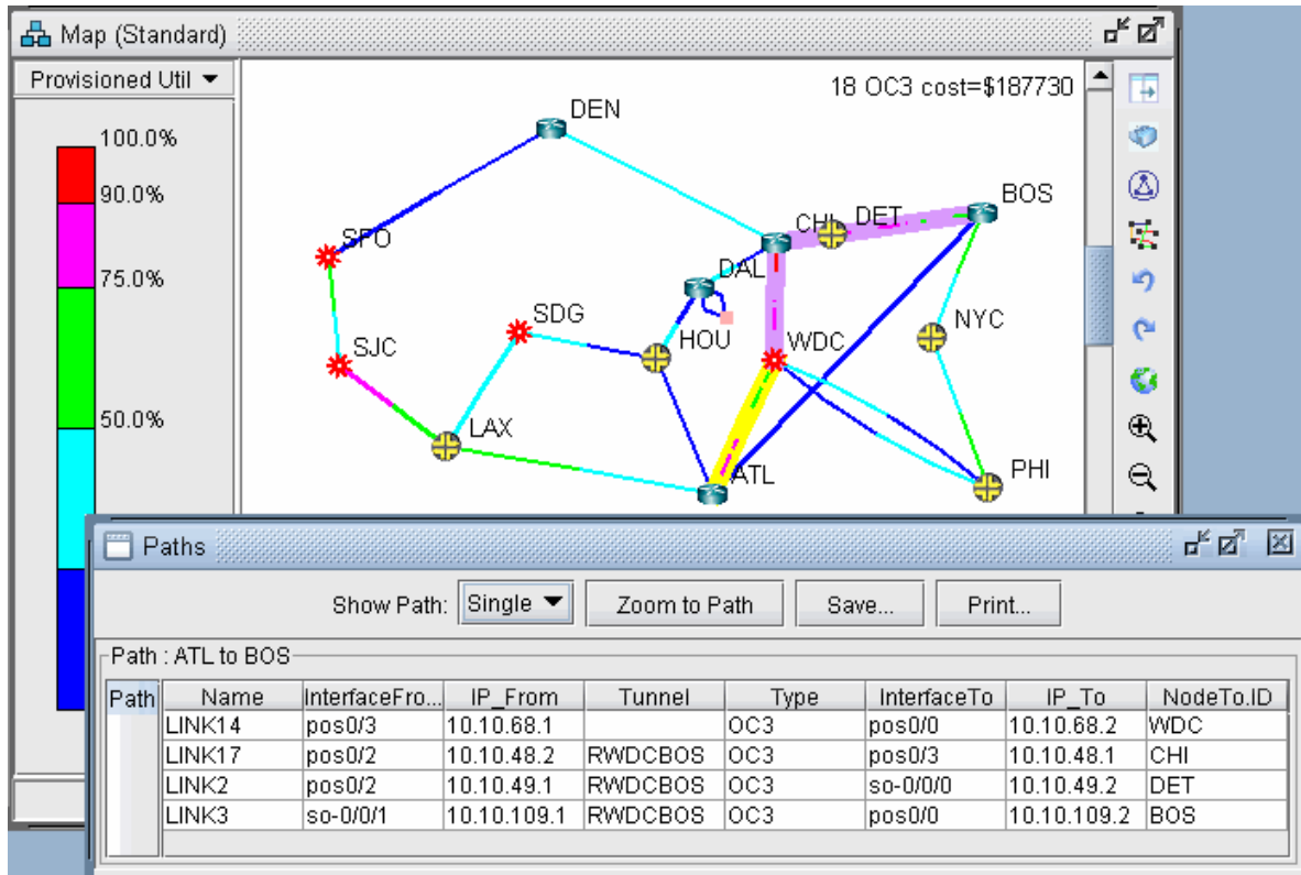
Figure 170: GRE Tunnel routed over LSP Tunnel
