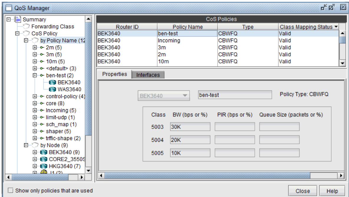
Figure 184: CoS Policy
