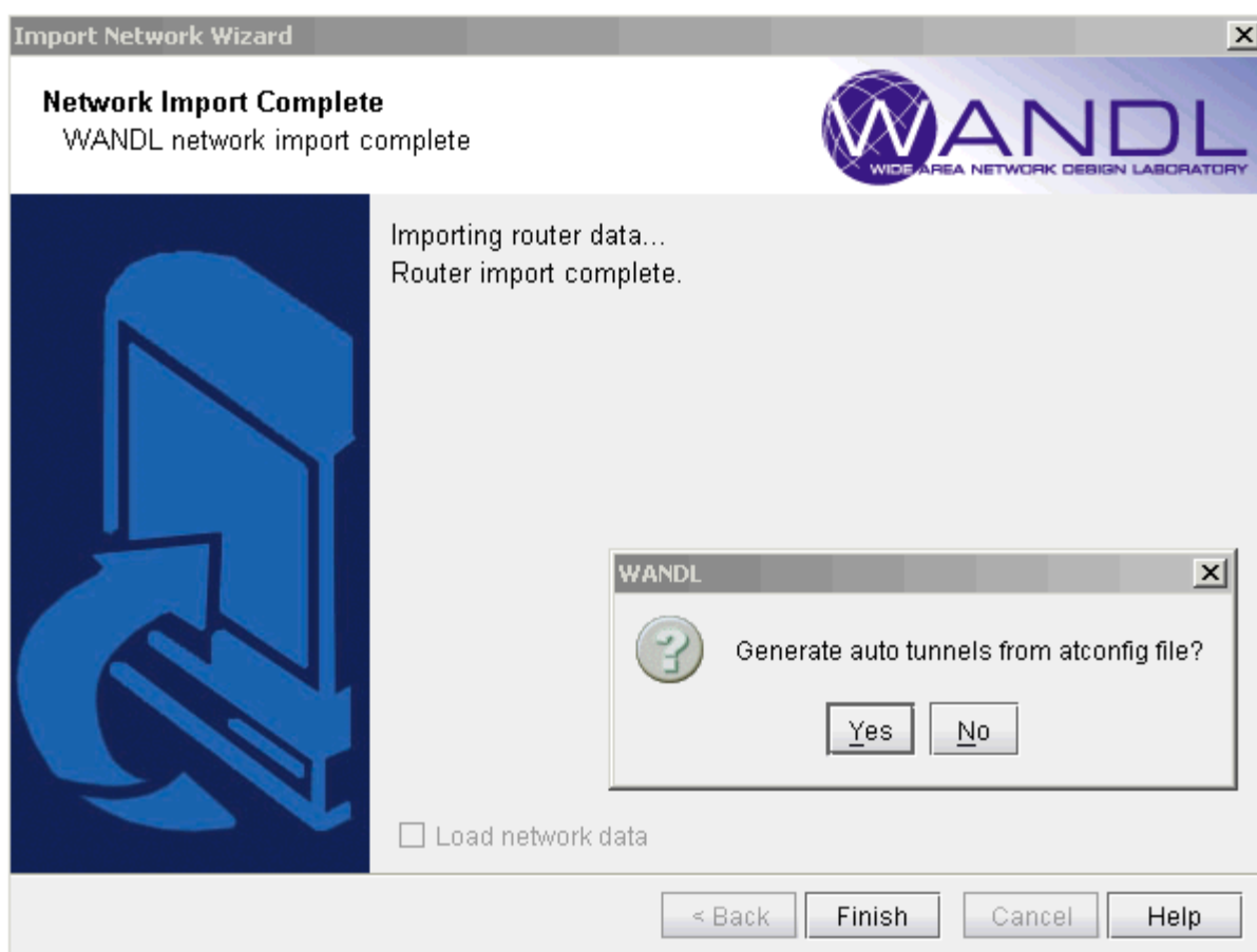
Figure 328: Configuration Import
