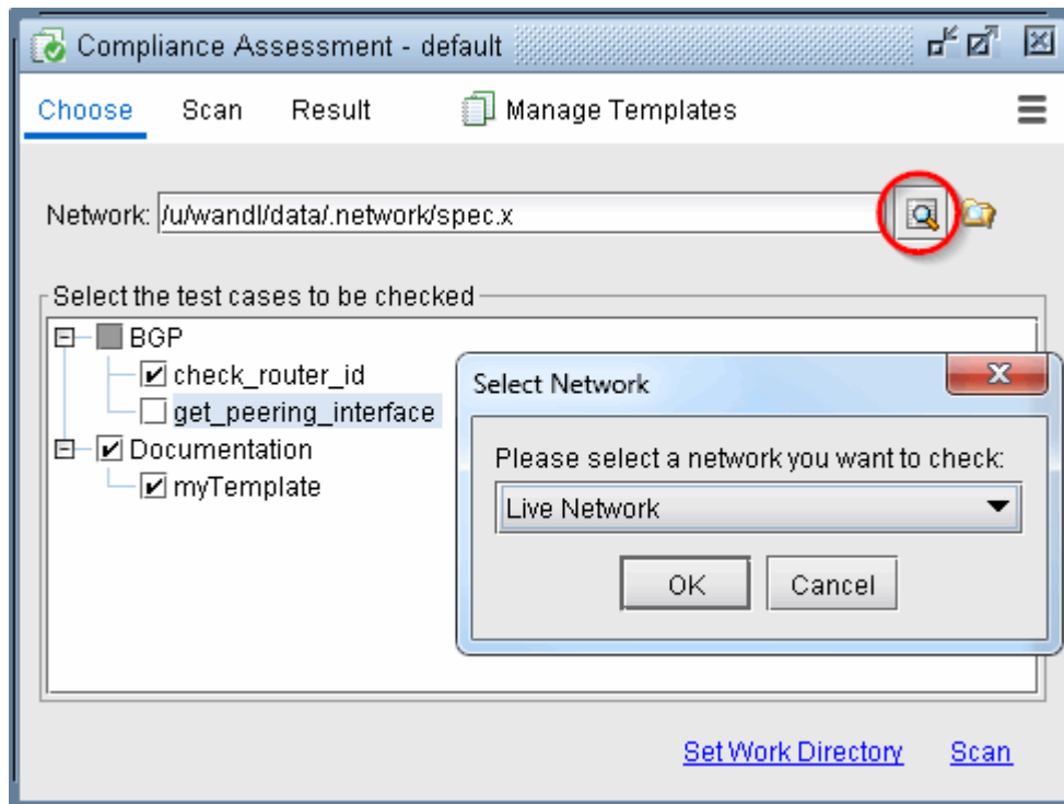
Figure 365: Choosing Network
