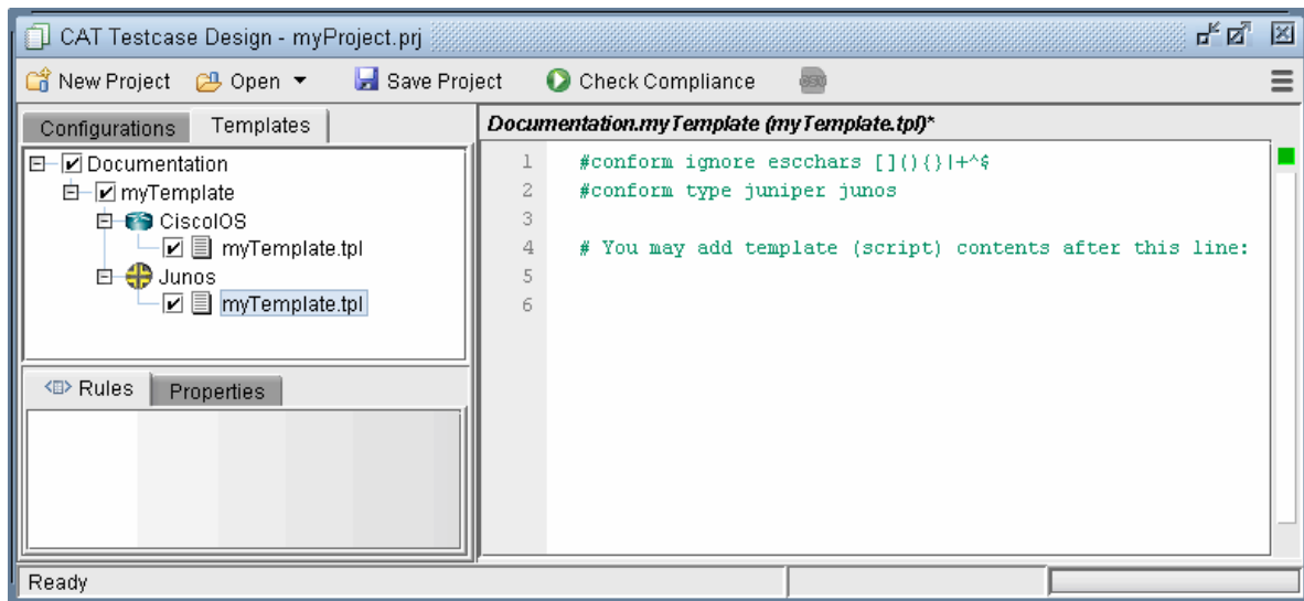
Figure 358: Initial Template
