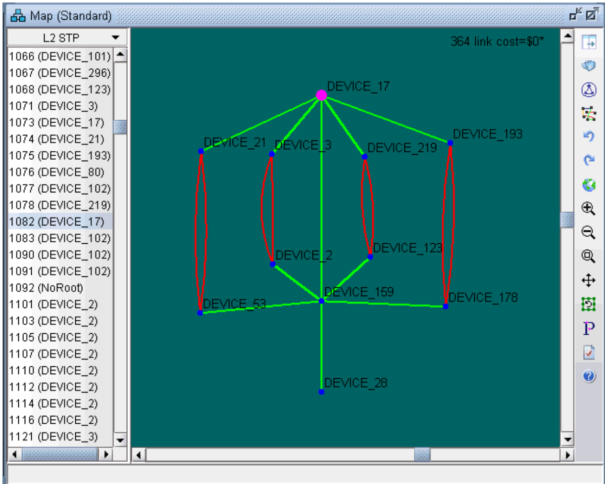
Figure 383: Topology View of a Spanning Tree
