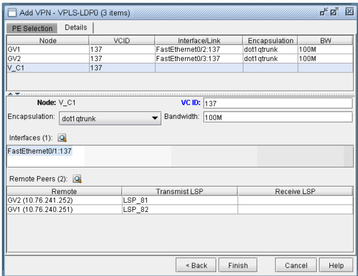
Figure 137: VPLS-LDP instance details configured
