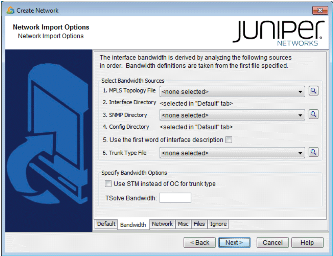
Figure 5: Bandwidth Tab
