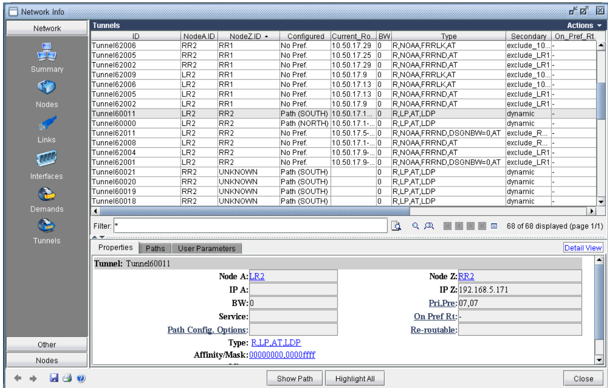
Figure 333: Tunnels Window Showing Only Auto-Tunnels
