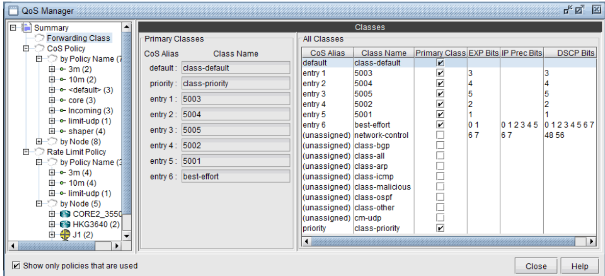
Figure 183: QoS Manager
