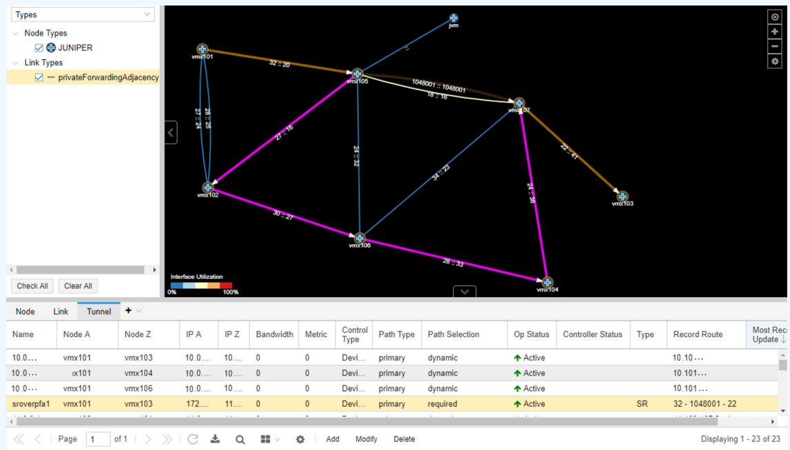
Figure 140: Reduced Label Stack Example
