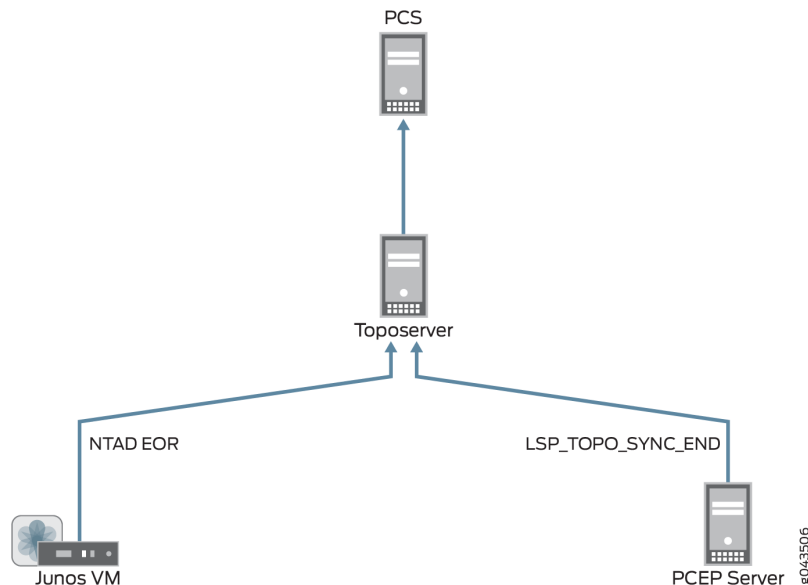
Figure 286: Model Updates Using Reset Network Model
