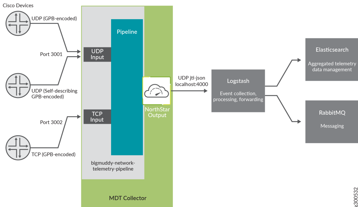
Figure 230: NorthStar MDT Collector Data Flow
