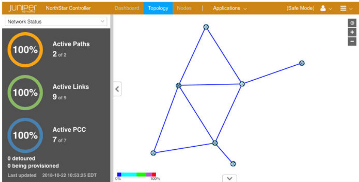
Figure 290: Fail-Safe Mode Landing Page
