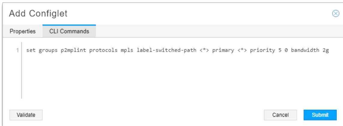
Figure 82: Add Configlet Window, CLI Example
