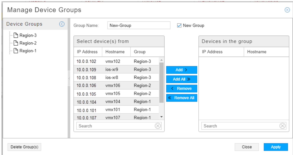
Figure 202: Manage Device Groups Window
