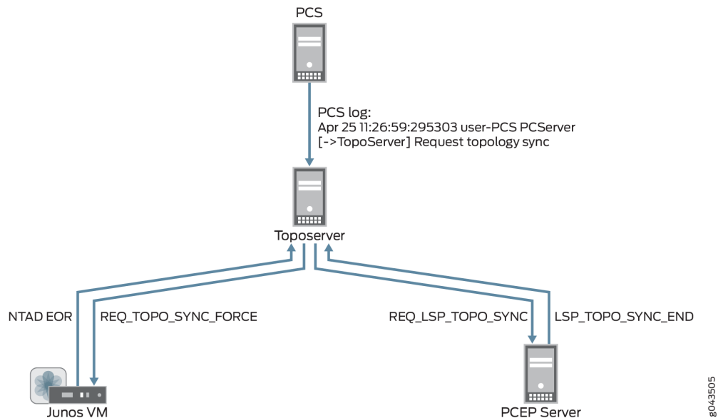
Figure 287: Synchronization Request and Model Updates Using Sync Network Model
