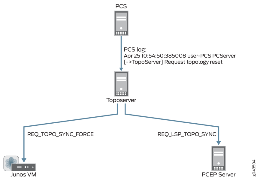
Figure 285: Reset Model Request
