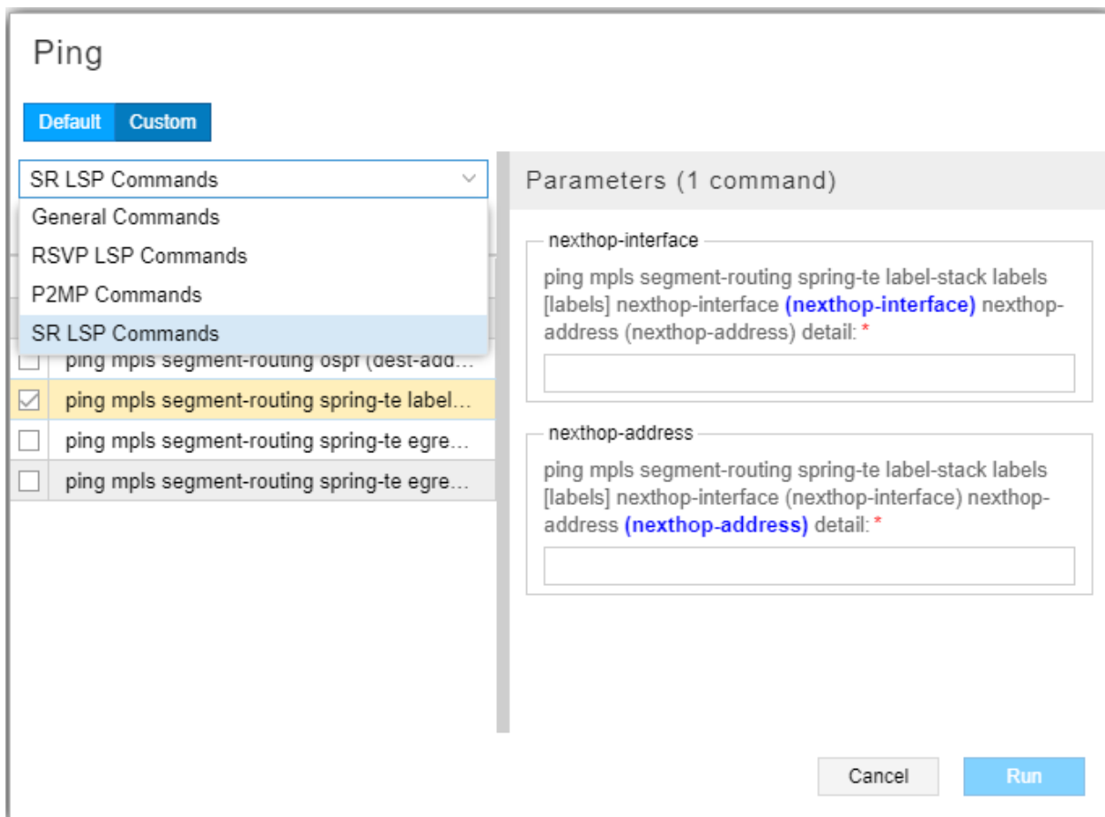
Figure 272: Ping Setup Window - Custom Tab
