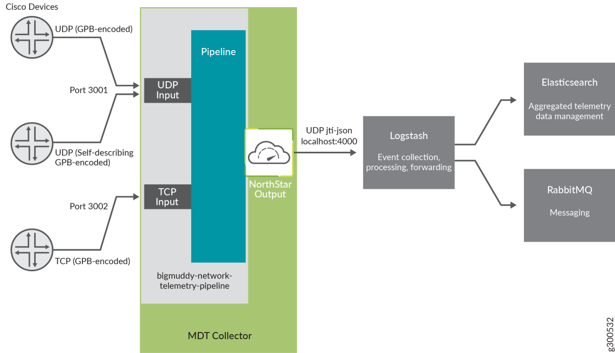
Figure 228: NorthStar MDT Collector Data Flow
