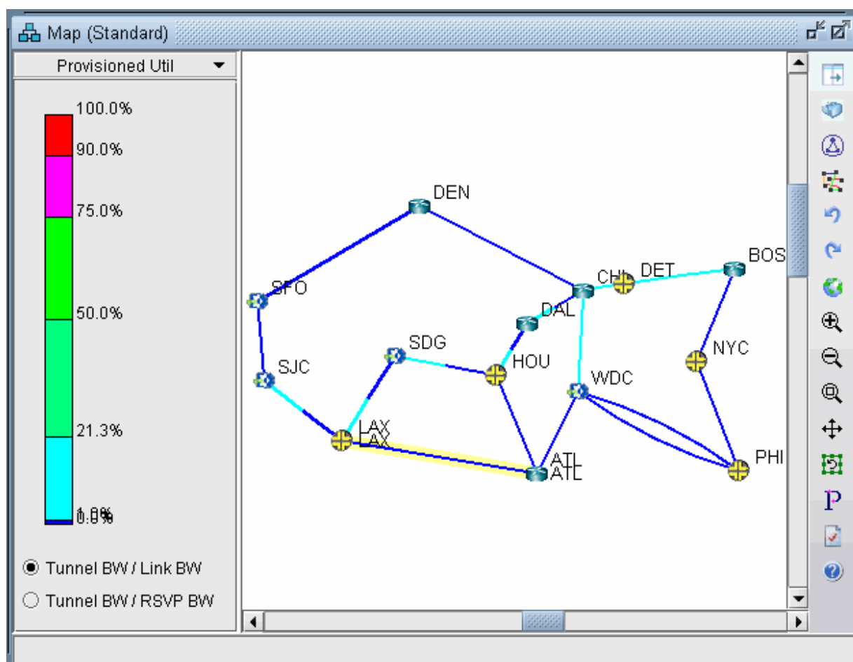
Figure 219: Planned Tunnel Utilization (Tunnel Layer View)
