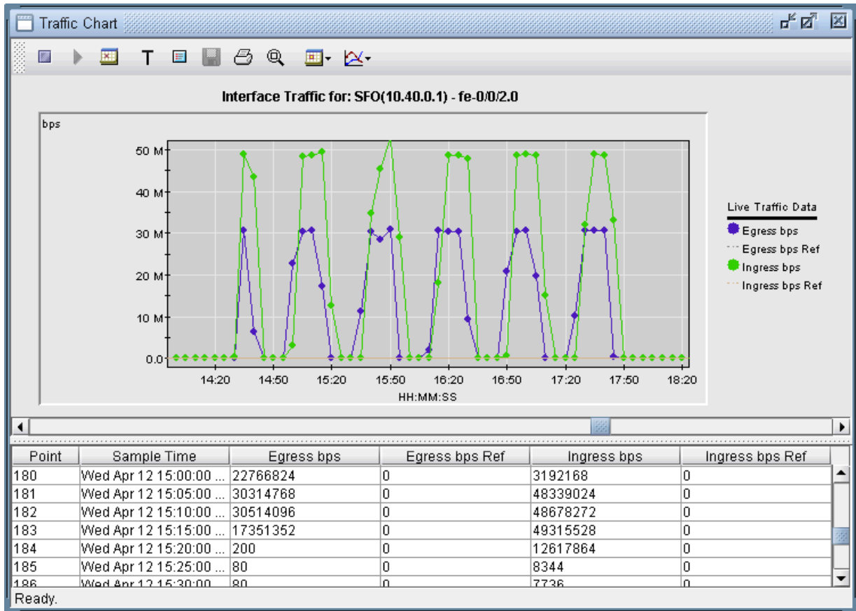
Figure 160: PE-&gt;CE Interface Traffic Chart (For PE Router SFO)
