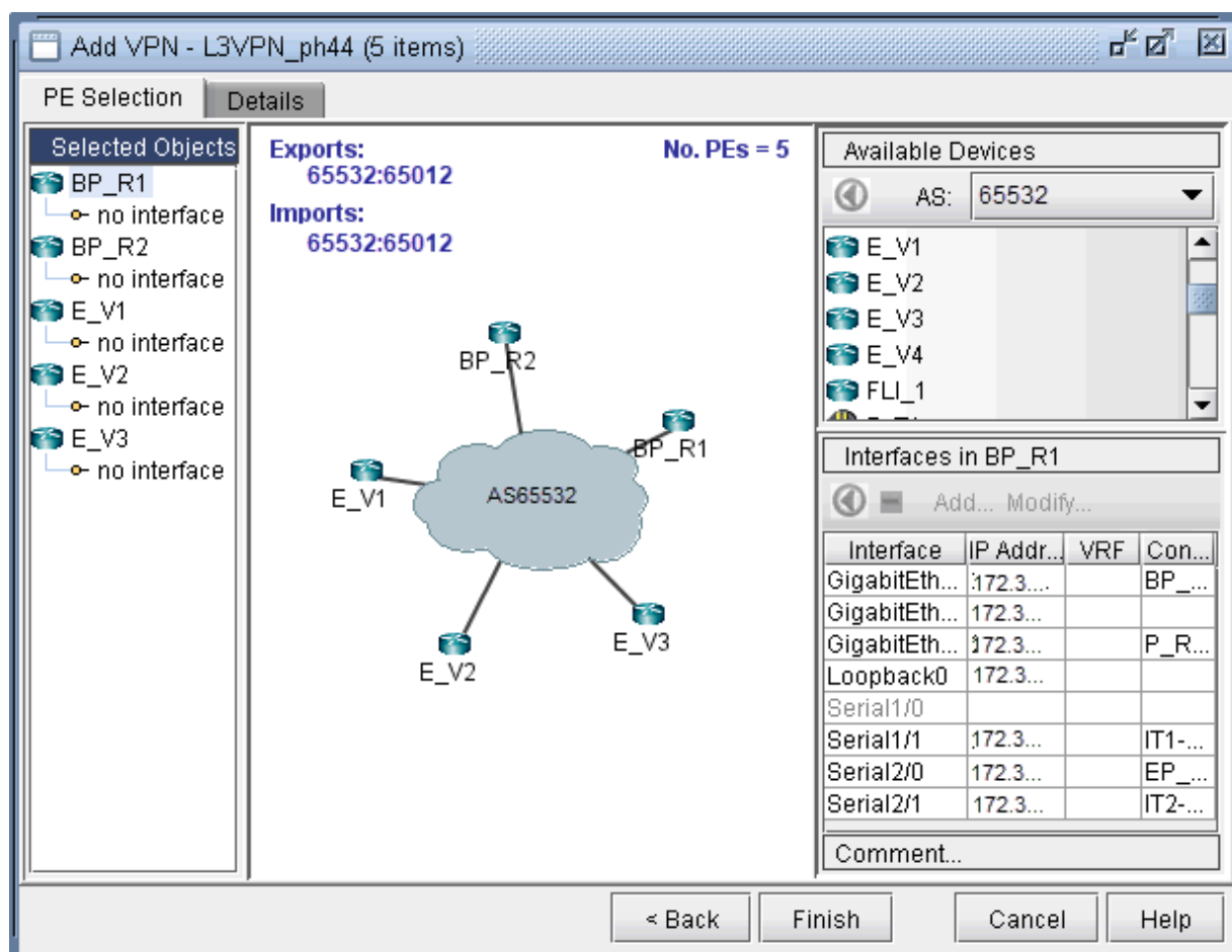
Figure 104: How to assign interfaces to PEs
