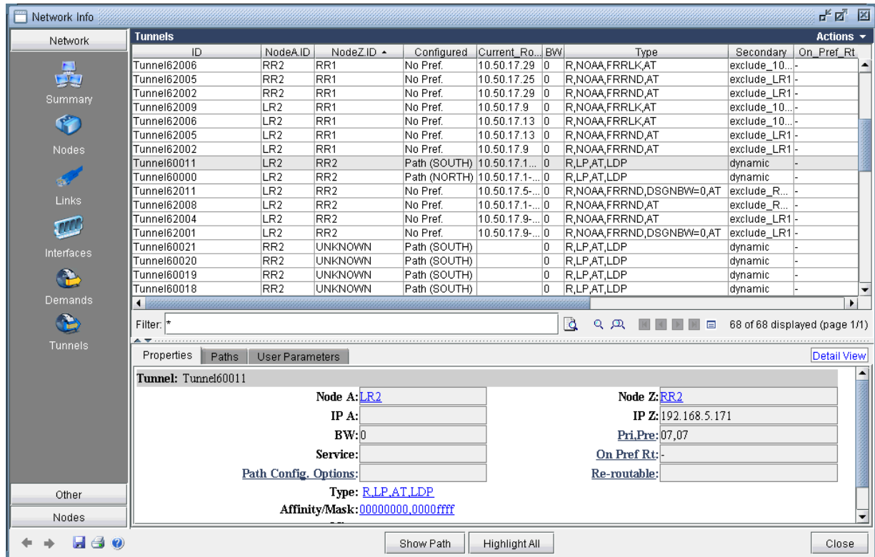
Figure 336: Tunnels Window Showing Only Auto-Tunnels
