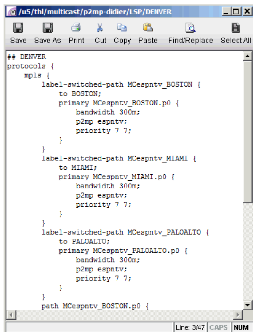
Figure 285: Configlet Generated for the P2MP LSP espntv.
