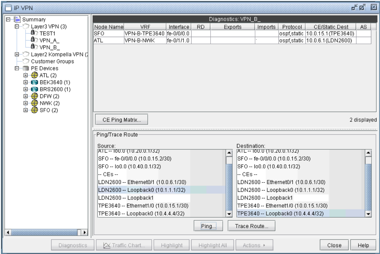
Figure 162: Ping/trace Route Between Routers from the IP VPN Window
