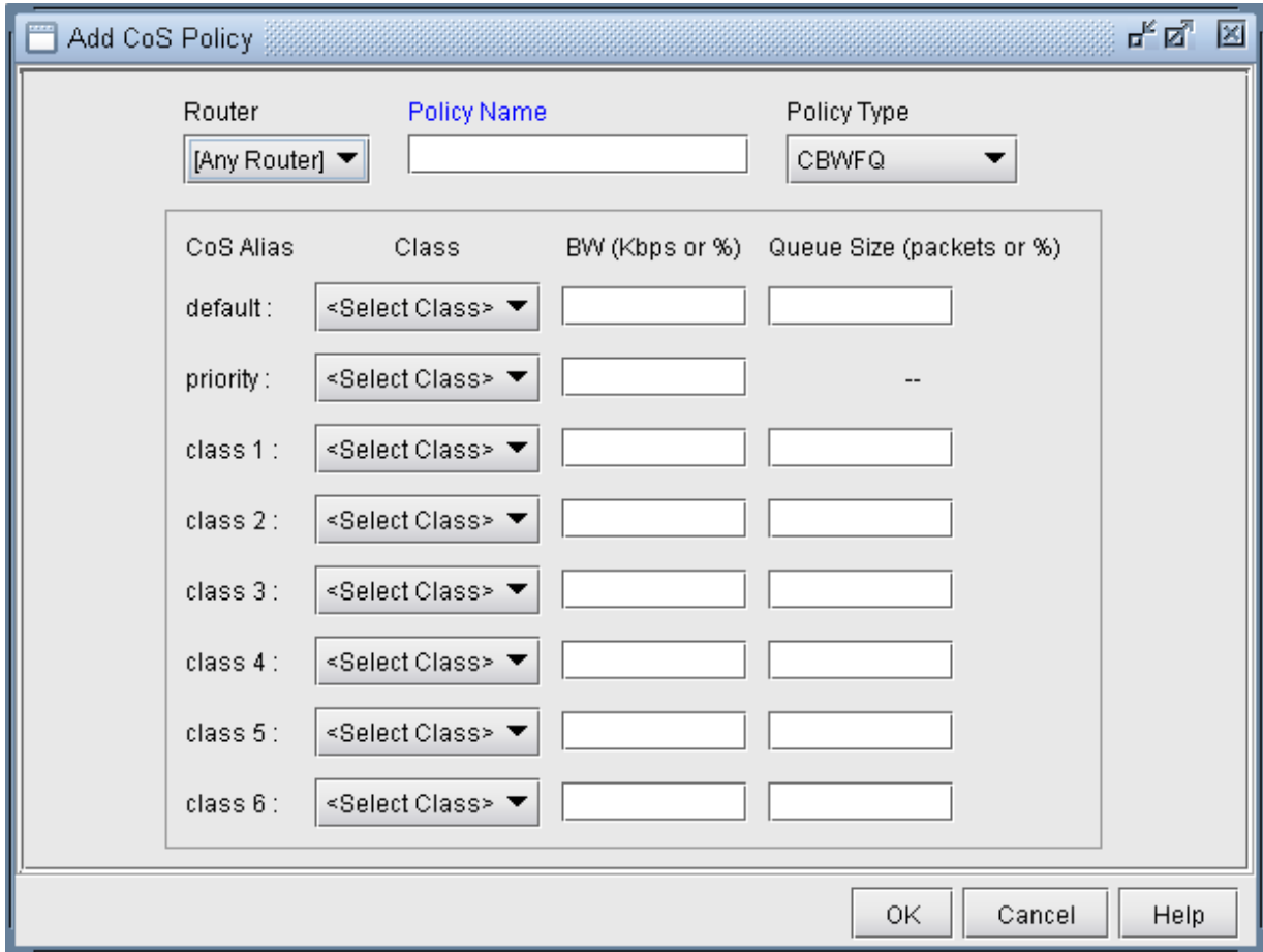
Figure 187: Add CoS Policy Window
